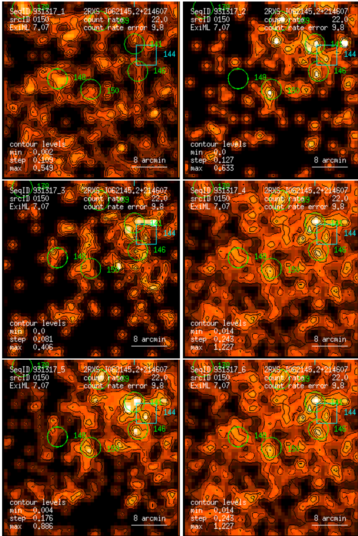
Figure 150: RASS 931317: detection 0150: band rate images, Gaussian filter: (1) PSPC channels 11 – 41, (2) 52 – 90, (3) 91 – 201, (4) 11 – 235, (5) 52 – 201, (6) 11 – 201. Broad band rates in counts/ks. Band rate contour levels in counts/ks/arcmin 2 .
