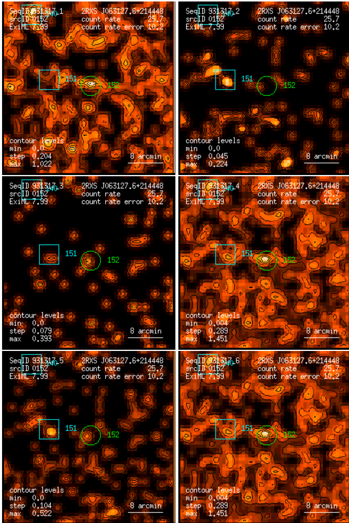
Figure 152: RASS 931317: detection 0152: band rate images, Gaussian filter: (1) PSPC channels 11 – 41, (2) 52 – 90, (3) 91 – 201, (4) 11 – 235, (5) 52 – 201, (6) 11 – 201. Broad band rates in counts/ks. Band rate contour levels in counts/ks/arcmin 2 .
