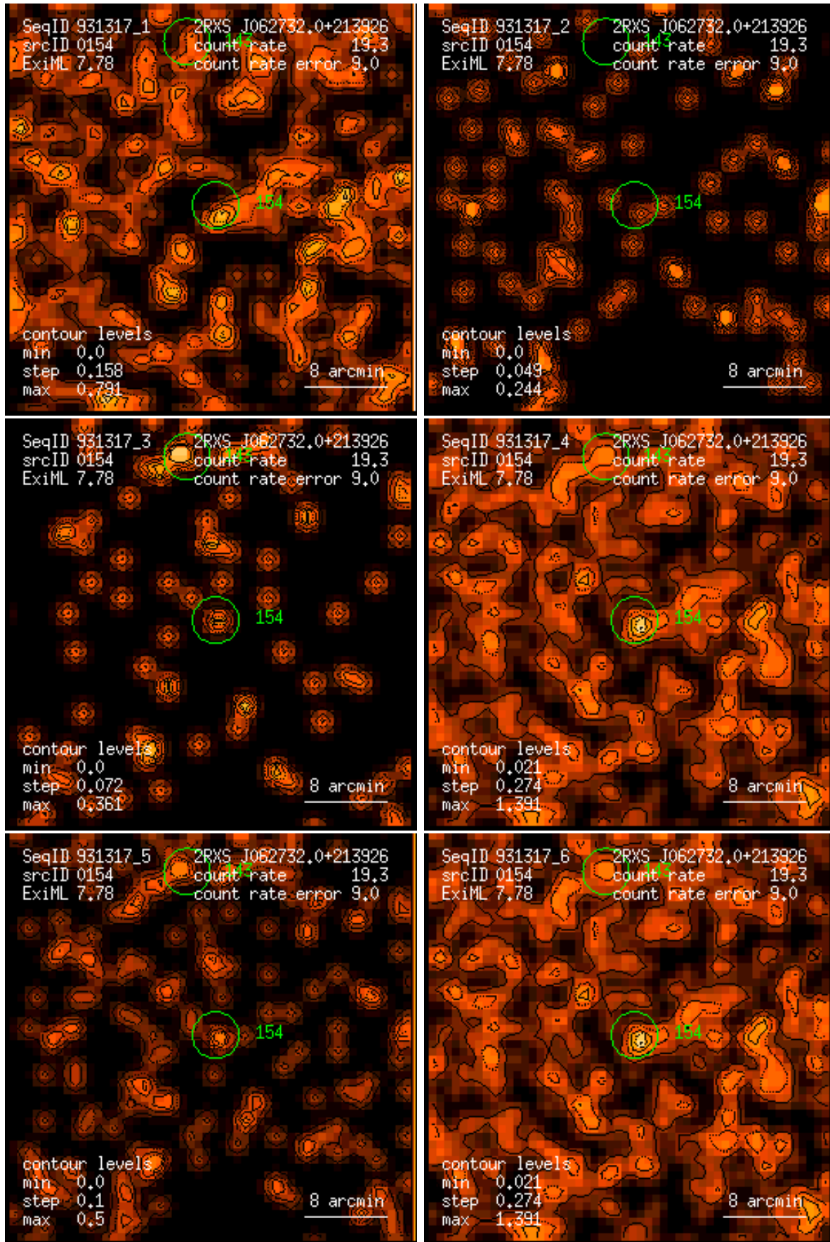
Figure 154: RASS 931317: detection 0154: band rate images, Gaussian filter: (1) PSPC channels 11 – 41, (2) 52 – 90, (3) 91 – 201, (4) 11 – 235, (5) 52 – 201, (6) 11 – 201. Broad band rates in counts/ks. Band rate contour levels in counts/ks/arcmin 2 .
