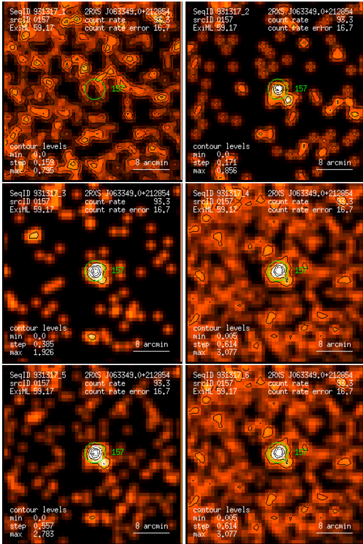
Figure 157: RASS 931317: detection 0157: band rate images, Gaussian filter: (1) PSPC channels 11 – 41, (2) 52 – 90, (3) 91 – 201, (4) 11 – 235, (5) 52 – 201, (6) 11 – 201. Broad band rates in counts/ks. Band rate contour levels in counts/ks/arcmin 2 .
