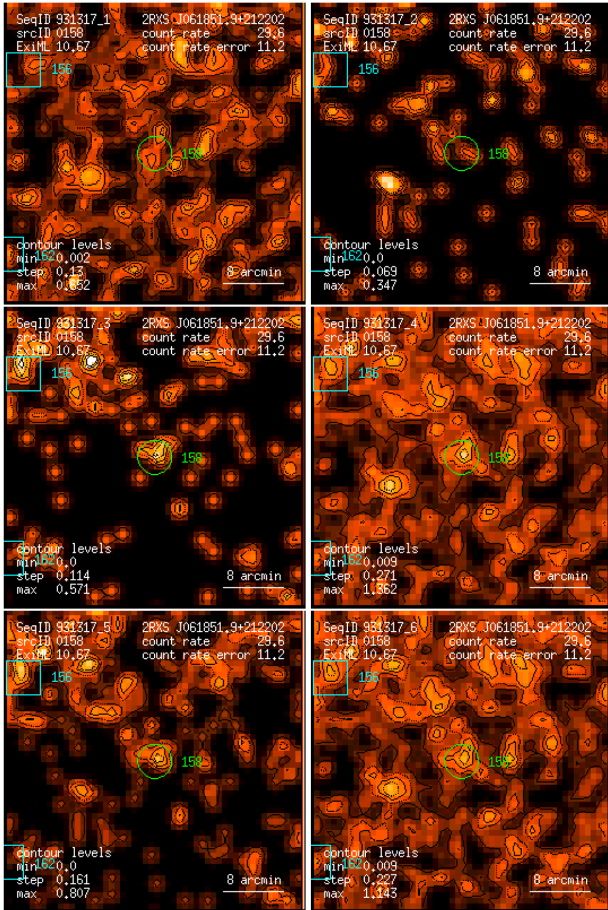
Figure 158: RASS 931317: detection 0158: band rate images, Gaussian filter: (1) PSPC channels 11 – 41, (2) 52 – 90, (3) 91 – 201, (4) 11 – 235, (5) 52 – 201, (6) 11 – 201. Broad band rates in counts/ks. Band rate contour levels in counts/ks/arcmin 2 .
