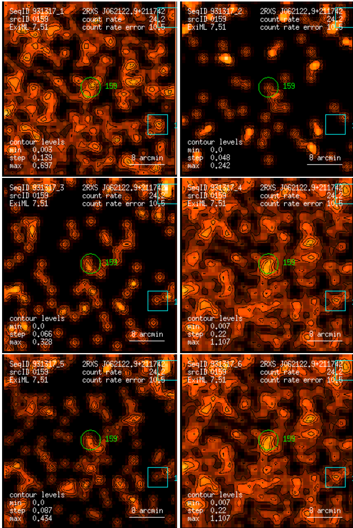
Figure 159: RASS 931317: detection 0159: band rate images, Gaussian filter: (1) PSPC channels 11 – 41, (2) 52 – 90, (3) 91 – 201, (4) 11 – 235, (5) 52 – 201, (6) 11 – 201. Broad band rates in counts/ks. Band rate contour levels in counts/ks/arcmin 2 .
