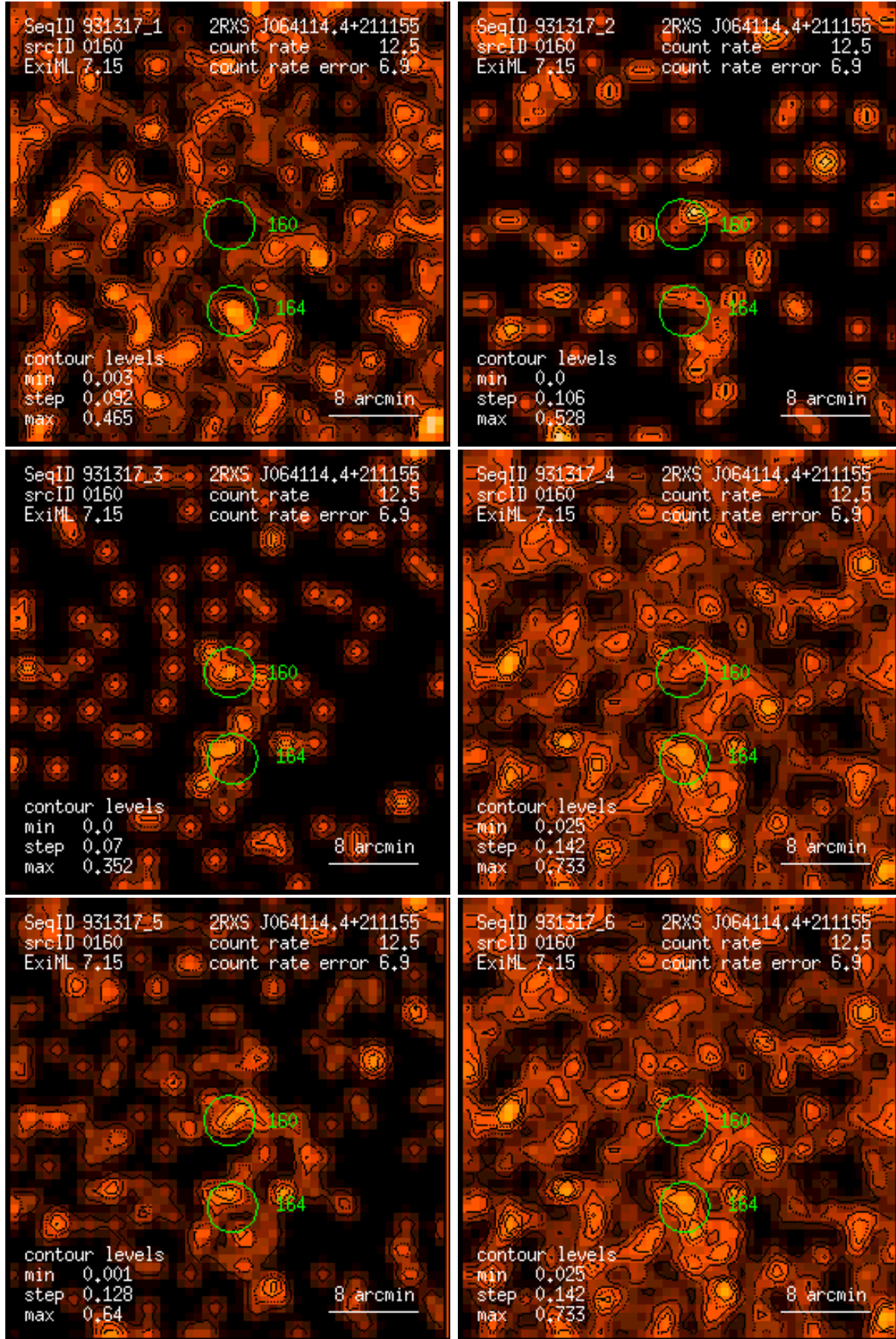
Figure 160: RASS 931317: detection 0160: band rate images, Gaussian filter: (1) PSPC channels 11 – 41, (2) 52 – 90, (3) 91 – 201, (4) 11 – 235, (5) 52 – 201, (6) 11 – 201. Broad band rates in counts/ks. Band rate contour levels in counts/ks/arcmin 2 .
