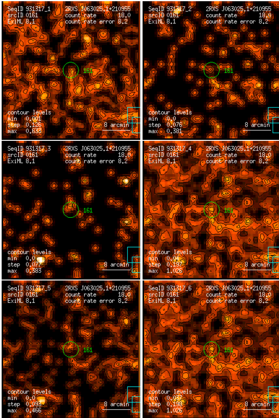
Figure 161: RASS 931317: detection 0161: band rate images, Gaussian filter: (1) PSPC channels 11 – 41, (2) 52 – 90, (3) 91 – 201, (4) 11 – 235, (5) 52 – 201, (6) 11 – 201. Broad band rates in counts/ks. Band rate contour levels in counts/ks/arcmin 2 .
