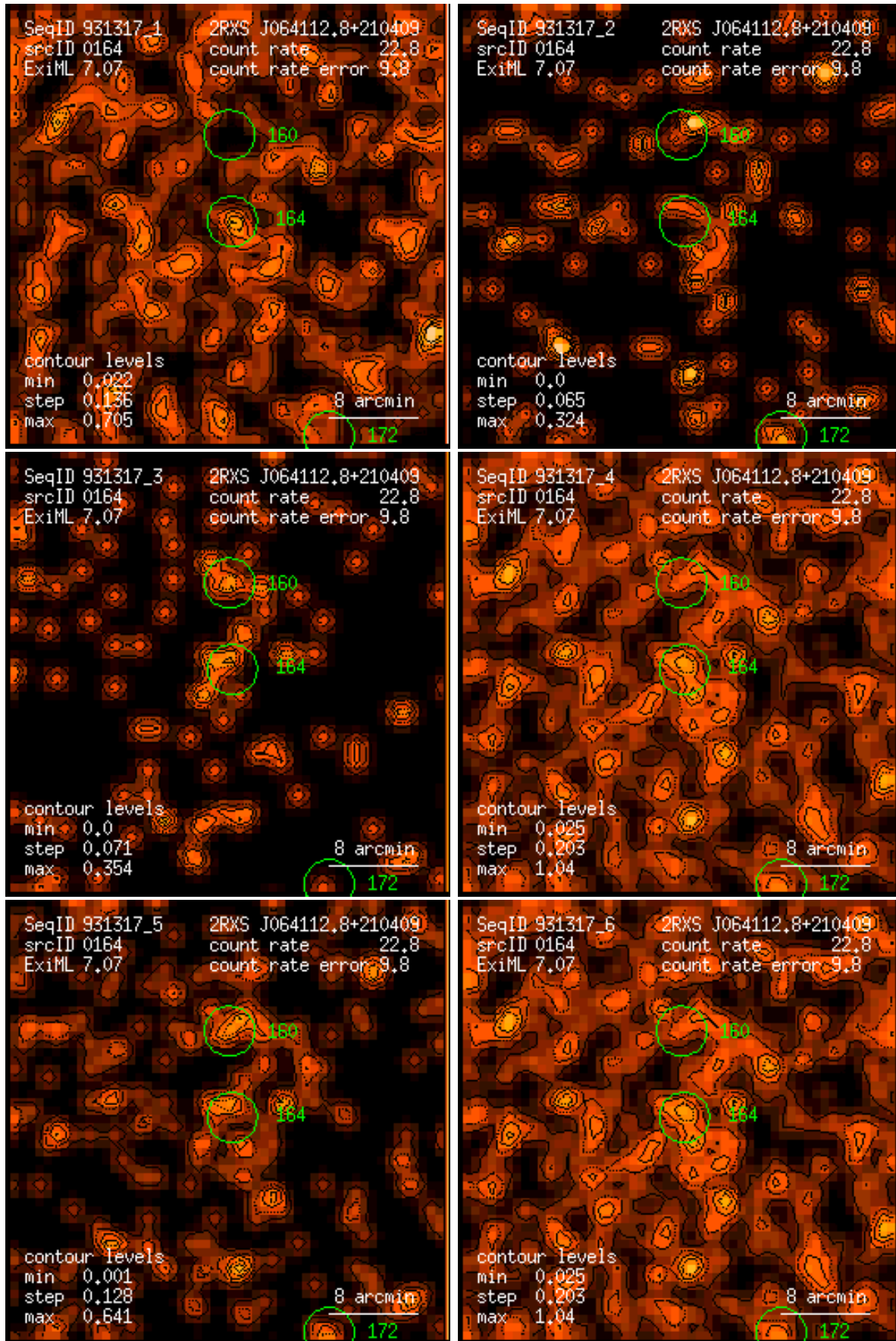
Figure 164: RASS 931317: detection 0164: band rate images, Gaussian filter: (1) PSPC channels 11 – 41, (2) 52 – 90, (3) 91 – 201, (4) 11 – 235, (5) 52 – 201, (6) 11 – 201. Broad band rates in counts/ks. Band rate contour levels in counts/ks/arcmin 2 .
