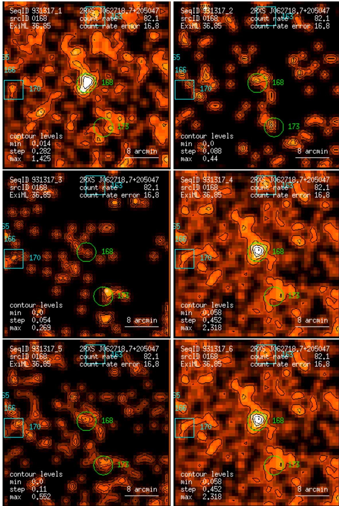
Figure 168: RASS 931317: detection 0168: band rate images, Gaussian filter: (1) PSPC channels 11 – 41, (2) 52 – 90, (3) 91 – 201, (4) 11 – 235, (5) 52 – 201, (6) 11 – 201. Broad band rates in counts/ks. Band rate contour levels in counts/ks/arcmin 2 .
