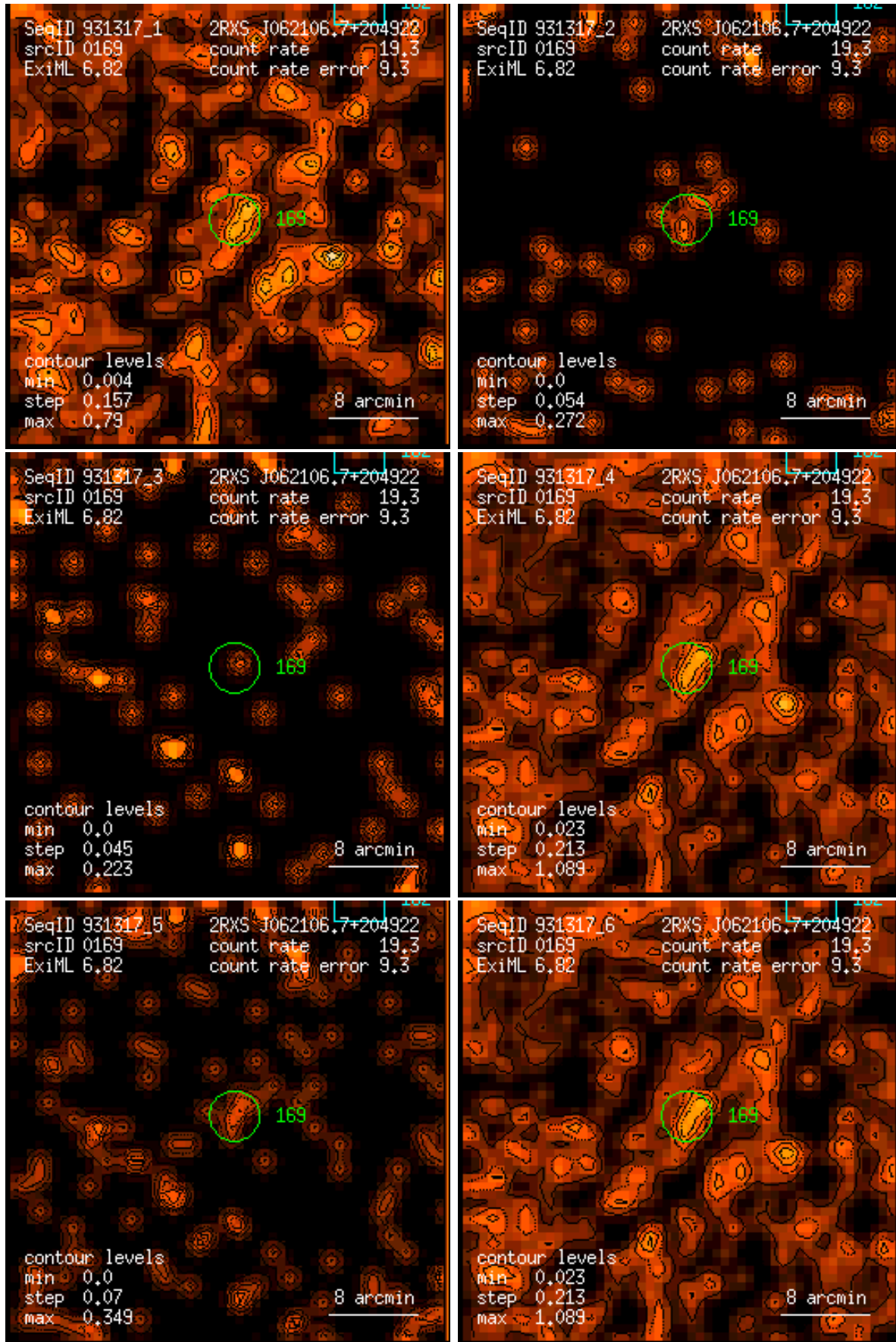
Figure 169: RASS 931317: detection 0169: band rate images, Gaussian filter: (1) PSPC channels 11 – 41, (2) 52 – 90, (3) 91 – 201, (4) 11 – 235, (5) 52 – 201, (6) 11 – 201. Broad band rates in counts/ks. Band rate contour levels in counts/ks/arcmin 2 .
