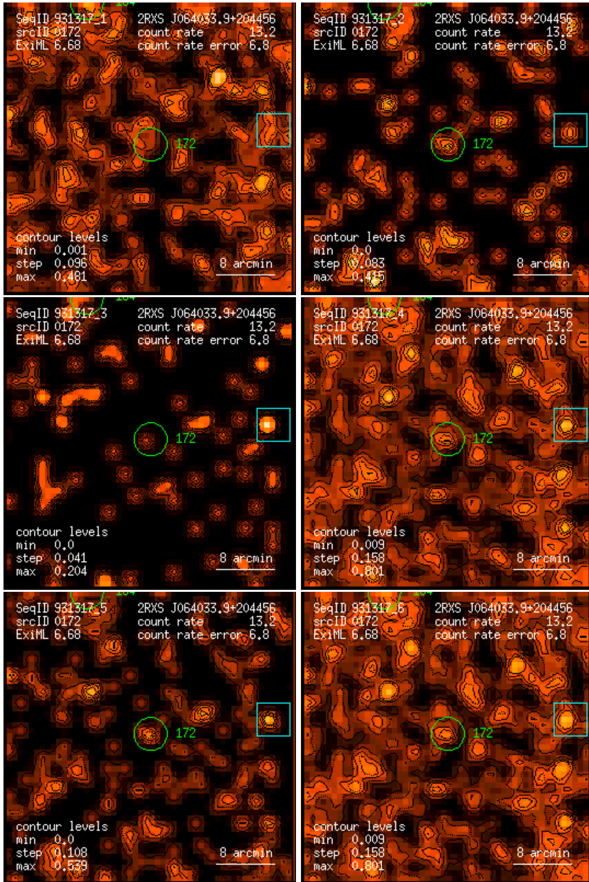
Figure 172: RASS 931317: detection 0172: band rate images, Gaussian filter: (1) PSPC channels 11 – 41, (2) 52 – 90, (3) 91 – 201, (4) 11 – 235, (5) 52 – 201, (6) 11 – 201. Broad band rates in counts/ks. Band rate contour levels in counts/ks/arcmin 2 .
