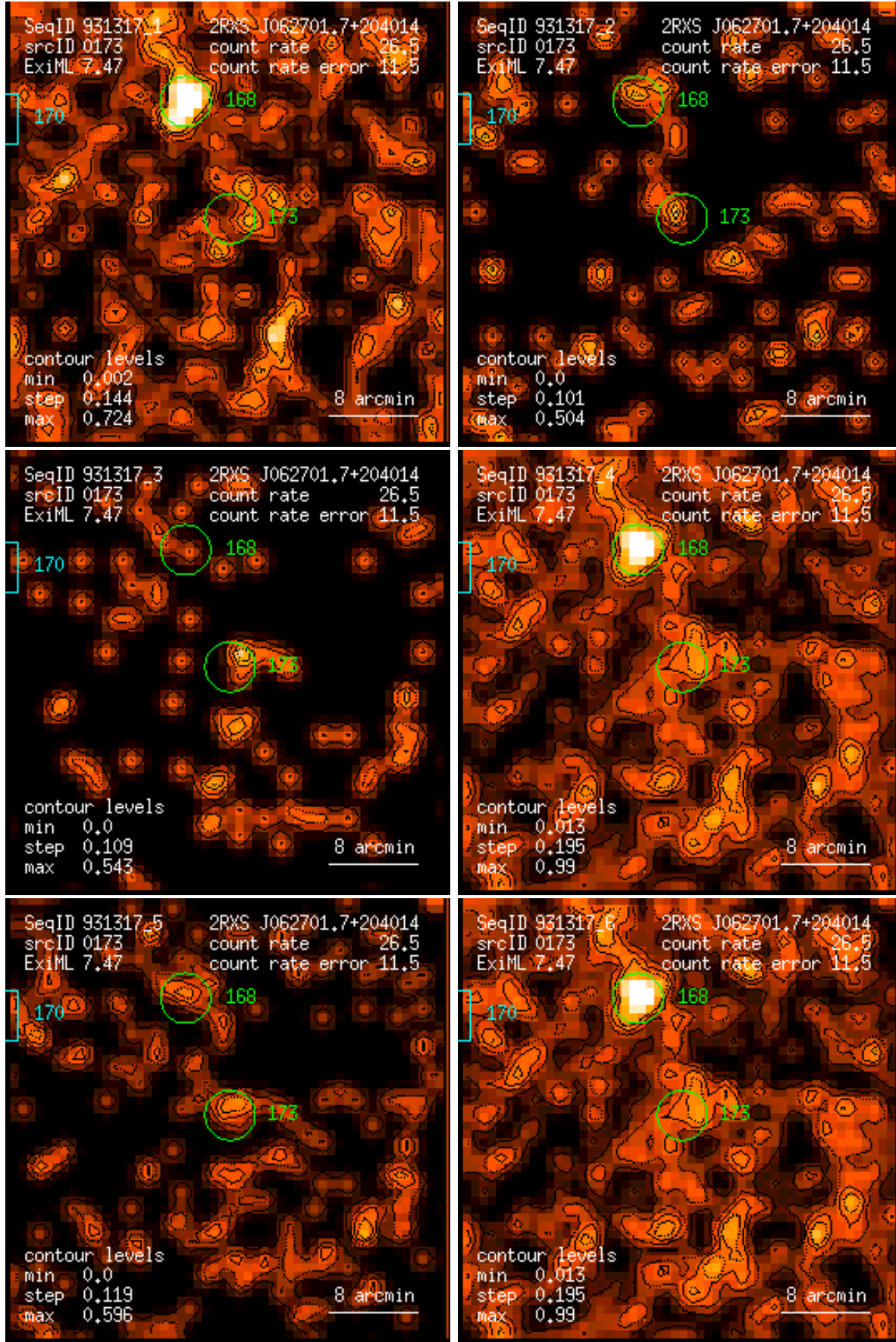
Figure 173: RASS 931317: detection 0173: band rate images, Gaussian filter: (1) PSPC channels 11 – 41, (2) 52 – 90, (3) 91 – 201, (4) 11 – 235, (5) 52 – 201, (6) 11 – 201. Broad band rates in counts/ks. Band rate contour levels in counts/ks/arcmin 2 .
