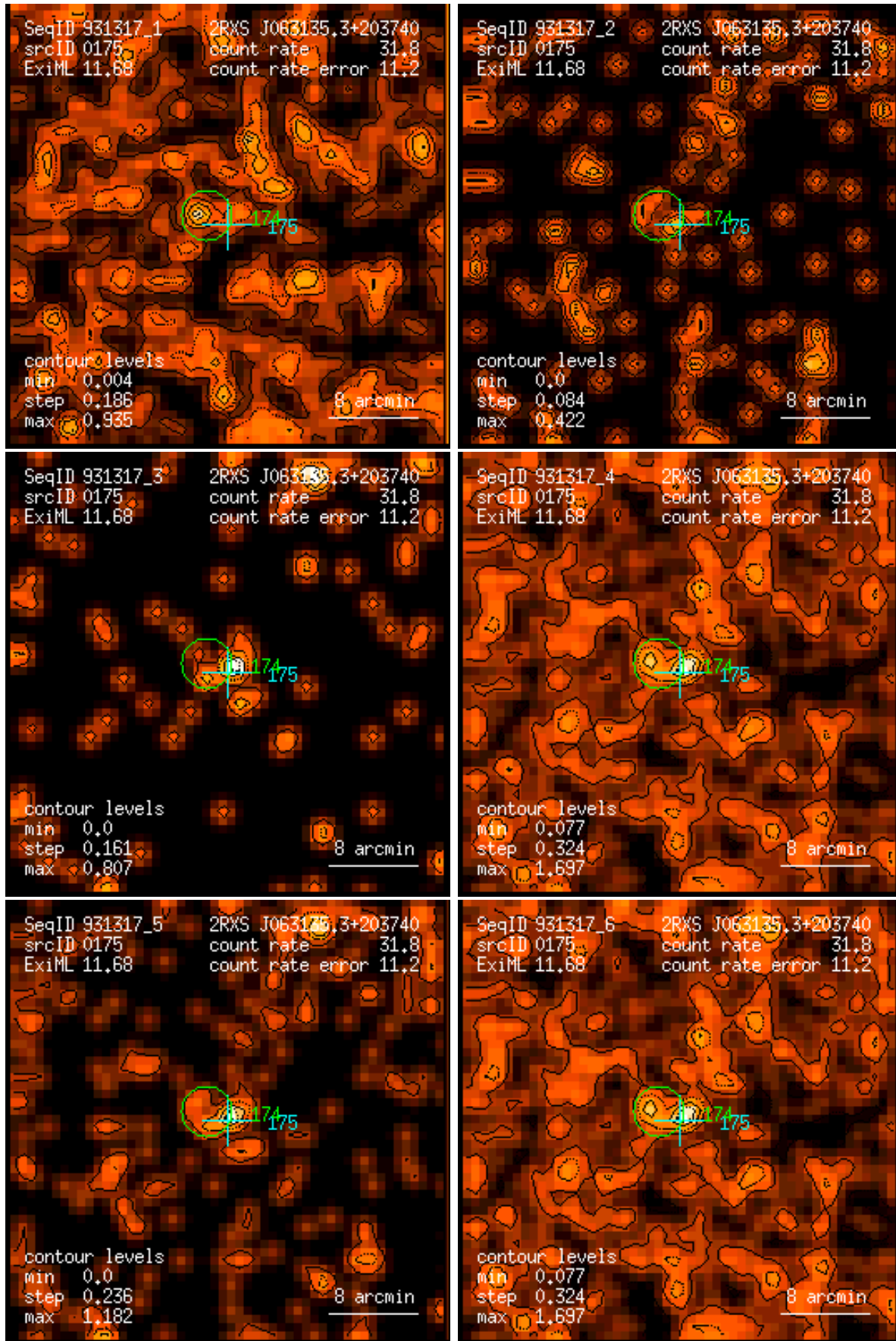
Figure 175: RASS 931317: detection 0175: band rate images, Gaussian filter: (1) PSPC channels 11 – 41, (2) 52 – 90, (3) 91 – 201, (4) 11 – 235, (5) 52 – 201, (6) 11 – 201. Broad band rates in counts/ks. Band rate contour levels in counts/ks/arcmin 2 .
