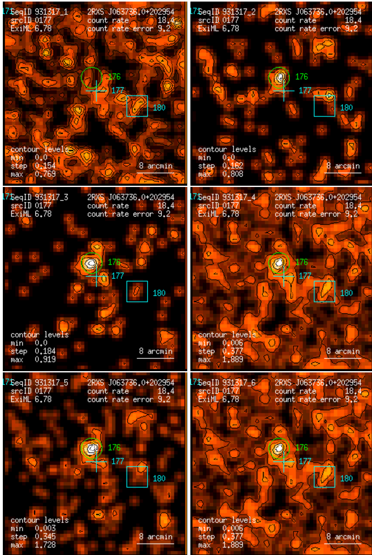
Figure 177: RASS 931317: detection 0177: band rate images, Gaussian filter: (1) PSPC channels 11 – 41, (2) 52 – 90, (3) 91 – 201, (4) 11 – 235, (5) 52 – 201, (6) 11 – 201. Broad band rates in counts/ks. Band rate contour levels in counts/ks/arcmin 2 .
