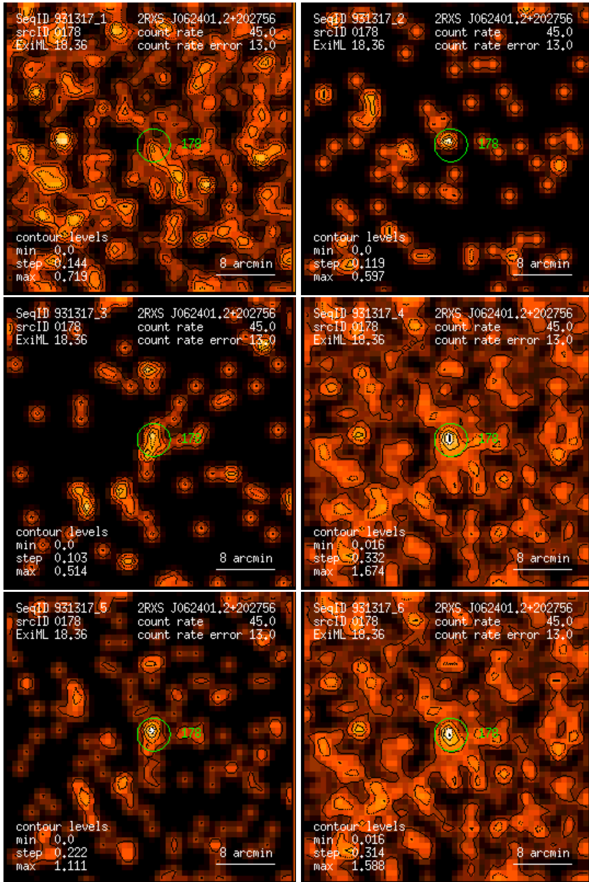
Figure 178: RASS 931317: detection 0178: band rate images, Gaussian filter: (1) PSPC channels 11 – 41, (2) 52 – 90, (3) 91 – 201, (4) 11 – 235, (5) 52 – 201, (6) 11 – 201. Broad band rates in counts/ks. Band rate contour levels in counts/ks/arcmin 2 .
