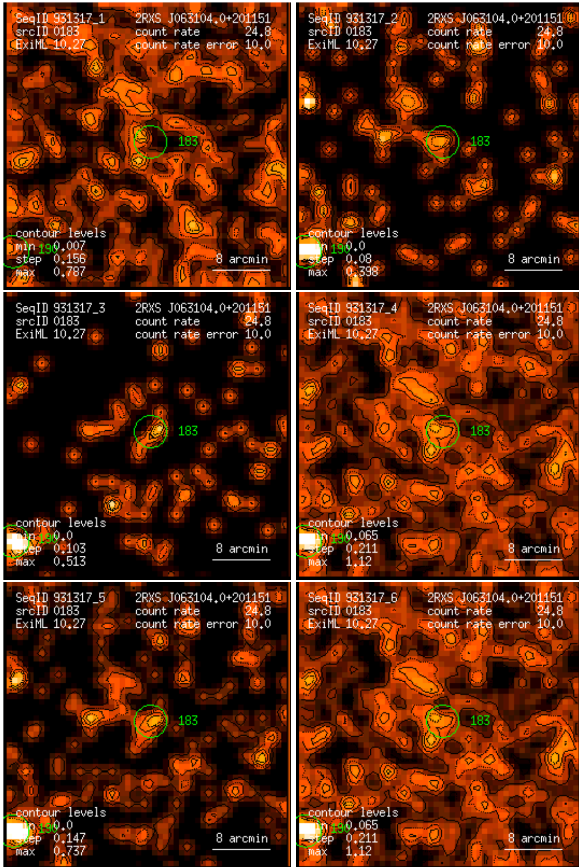
Figure 183: RASS 931317: detection 0183: band rate images, Gaussian filter: (1) PSPC channels 11 – 41, (2) 52 – 90, (3) 91 – 201, (4) 11 – 235, (5) 52 – 201, (6) 11 – 201. Broad band rates in counts/ks. Band rate contour levels in counts/ks/arcmin 2 .
