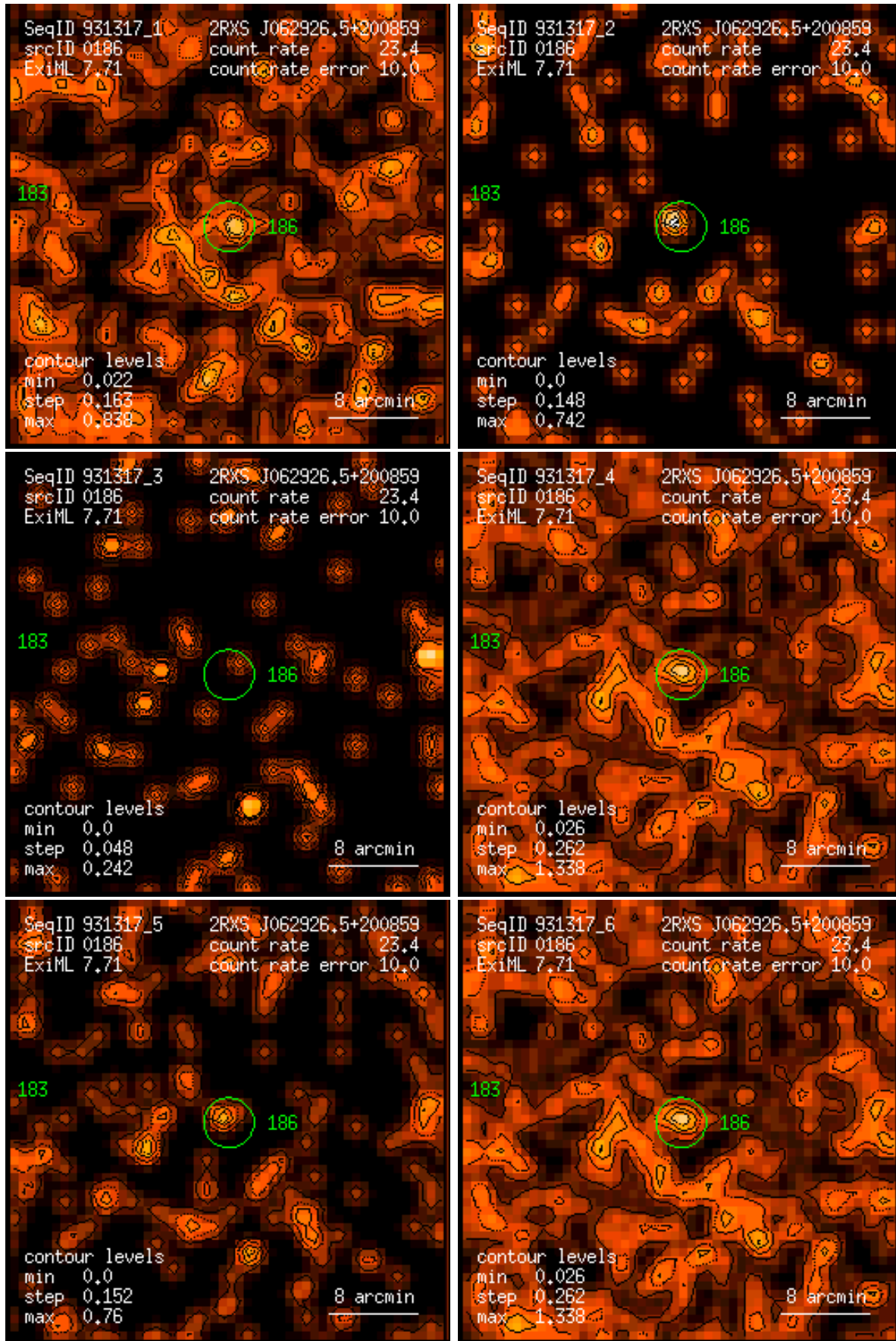
Figure 186: RASS 931317: detection 0186: band rate images, Gaussian filter: (1) PSPC channels 11 – 41, (2) 52 – 90, (3) 91 – 201, (4) 11 – 235, (5) 52 – 201, (6) 11 – 201. Broad band rates in counts/ks. Band rate contour levels in counts/ks/arcmin 2 .
