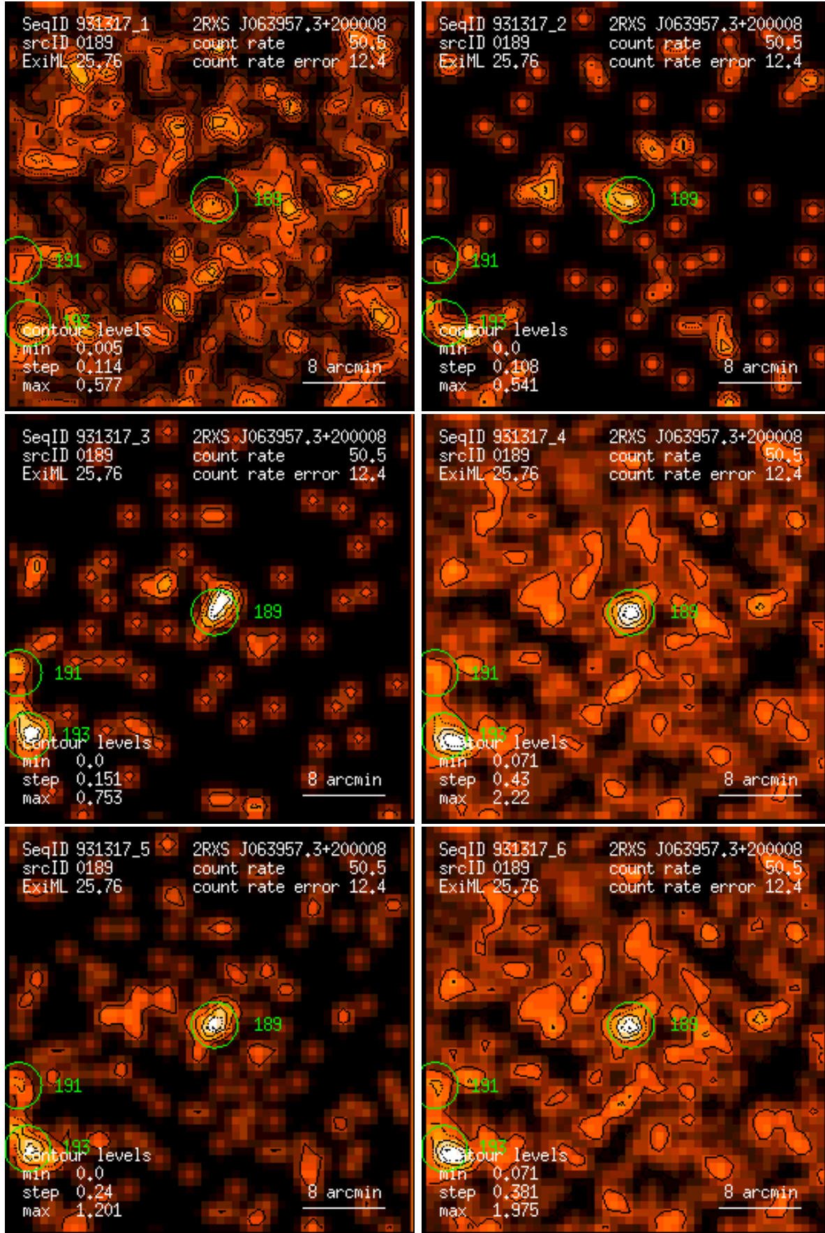
Figure 189: RASS 931317: detection 0189: band rate images, Gaussian filter: (1) PSPC channels 11 – 41, (2) 52 – 90, (3) 91 – 201, (4) 11 – 235, (5) 52 – 201, (6) 11 – 201. Broad band rates in counts/ks. Band rate contour levels in counts/ks/arcmin 2 .
