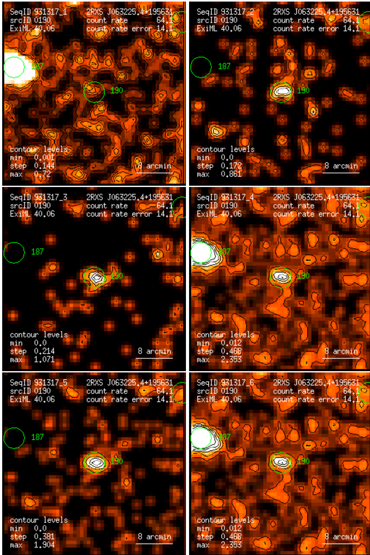
Figure 190: RASS 931317: detection 0190: band rate images, Gaussian filter: (1) PSPC channels 11 – 41, (2) 52 – 90, (3) 91 – 201, (4) 11 – 235, (5) 52 – 201, (6) 11 – 201. Broad band rates in counts/ks. Band rate contour levels in counts/ks/arcmin 2 .
