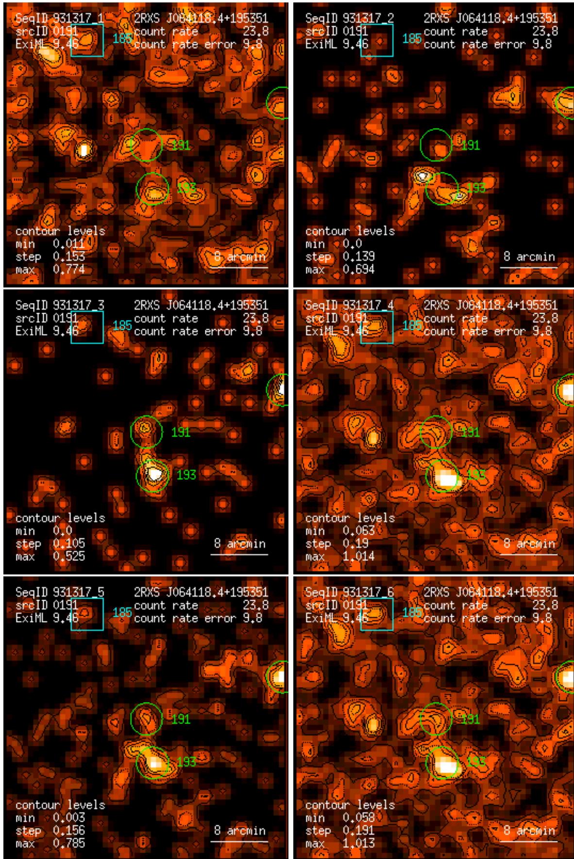
Figure 191: RASS 931317: detection 0191: band rate images, Gaussian filter: (1) PSPC channels 11 – 41, (2) 52 – 90, (3) 91 – 201, (4) 11 – 235, (5) 52 – 201, (6) 11 – 201. Broad band rates in counts/ks. Band rate contour levels in counts/ks/arcmin 2 .
