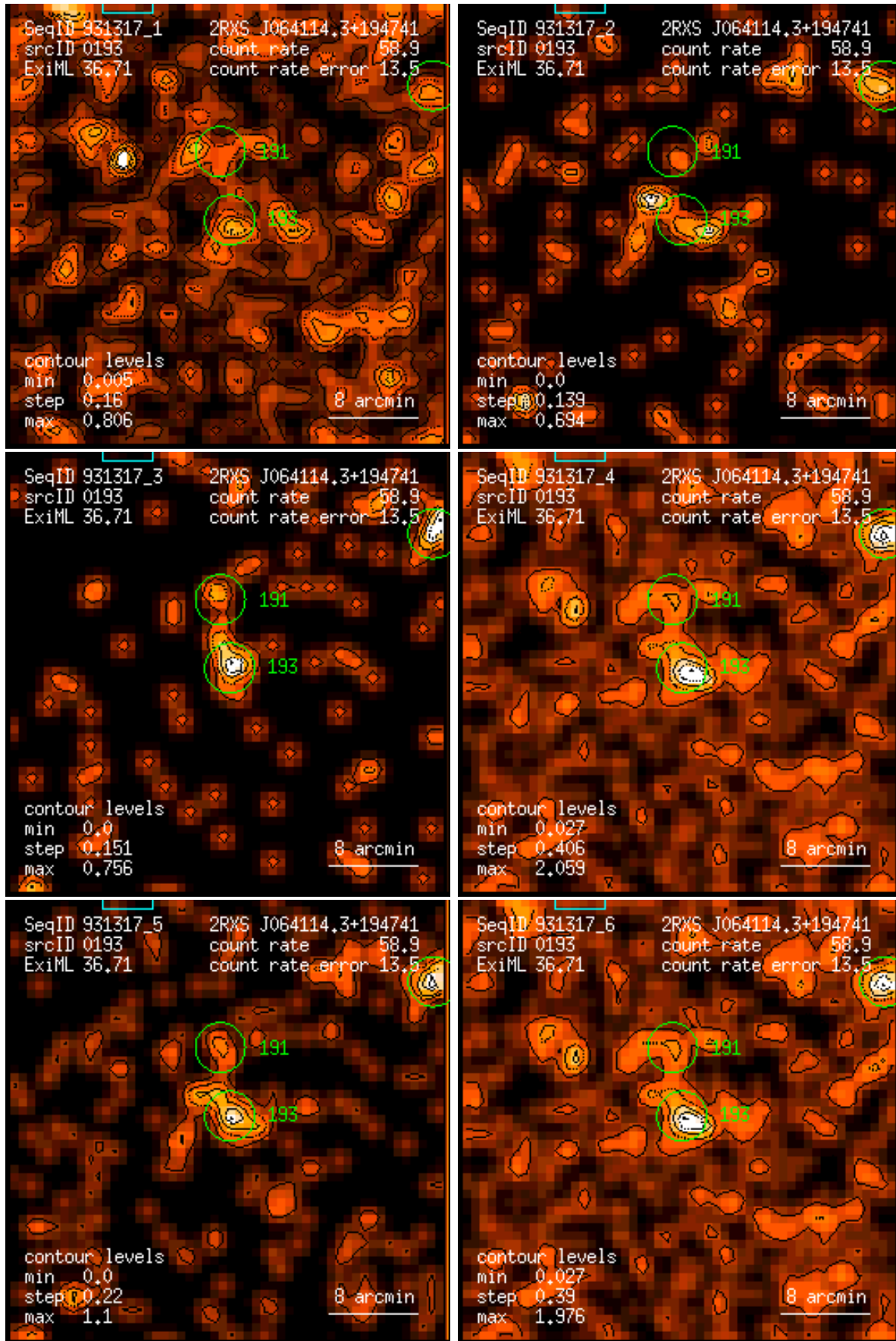
Figure 193: RASS 931317: detection 0193: band rate images, Gaussian filter: (1) PSPC channels 11 – 41, (2) 52 – 90, (3) 91 – 201, (4) 11 – 235, (5) 52 – 201, (6) 11 – 201. Broad band rates in counts/ks. Band rate contour levels in counts/ks/arcmin 2 .
