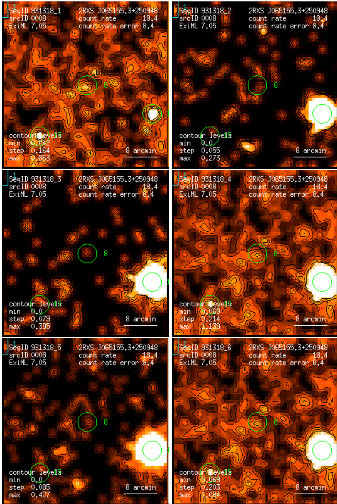
Figure 8: RASS 931318: detection 0008: band rate images, Gaussian filter: (1) PSPC channels 11 – 41, (2) 52 – 90, (3) 91 – 201, (4) 11 – 235, (5) 52 – 201, (6) 11 – 201. Broad band rates in counts/ks. Band rate contour levels in counts/ks/arcmin 2 .
