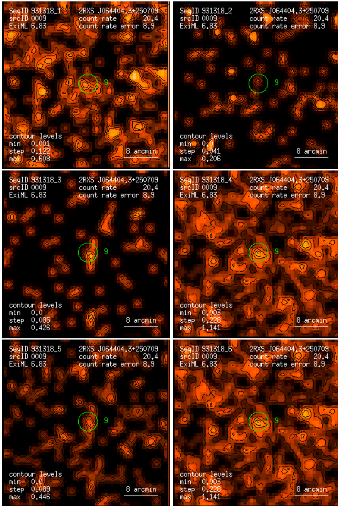
Figure 9: RASS 931318: detection 0009: band rate images, Gaussian filter: (1) PSPC channels 11 – 41, (2) 52 – 90, (3) 91 – 201, (4) 11 – 235, (5) 52 – 201, (6) 11 – 201. Broad band rates in counts/ks. Band rate contour levels in counts/ks/arcmin 2 .
