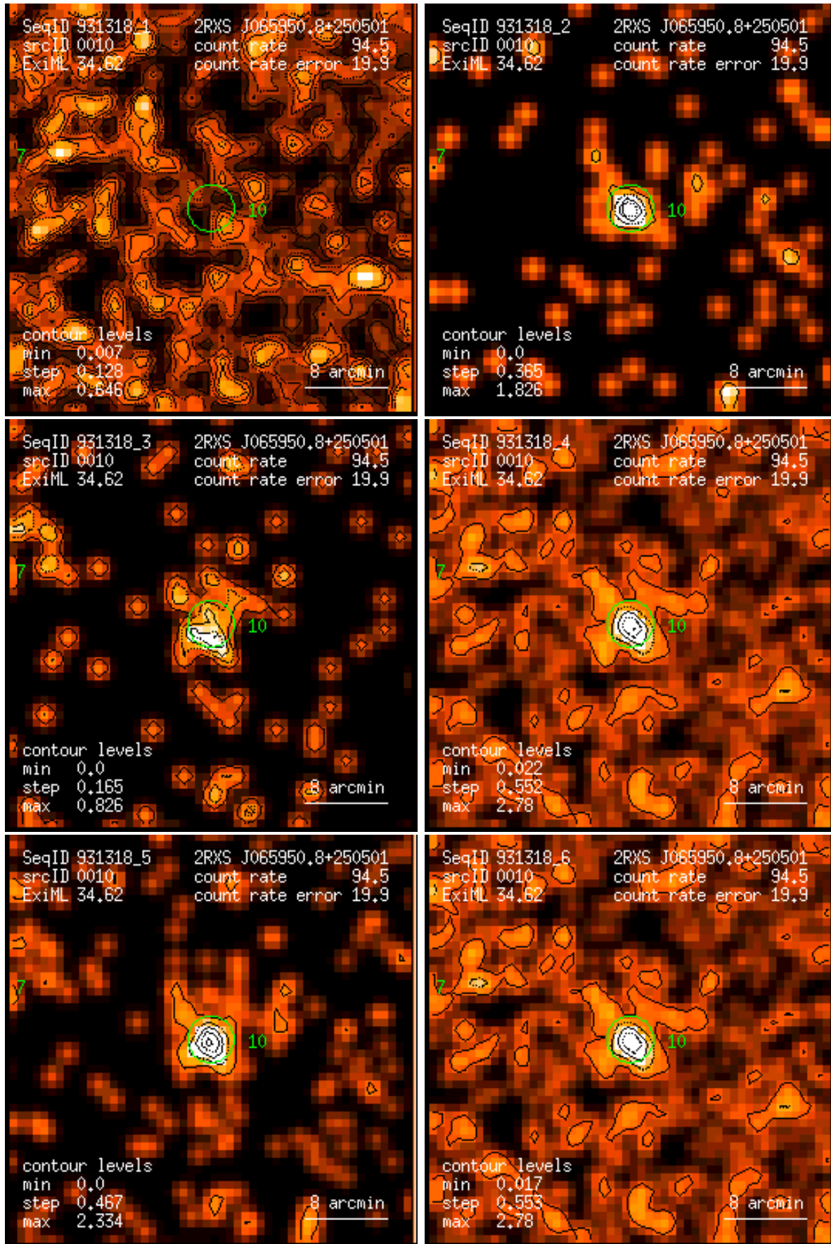
Figure 10: RASS 931318: detection 0010: band rate images, Gaussian filter: (1) PSPC channels 11 – 41, (2) 52 – 90, (3) 91 – 201, (4) 11 – 235, (5) 52 – 201, (6) 11 – 201. Broad band rates in counts/ks. Band rate contour levels in counts/ks/arcmin 2 .
