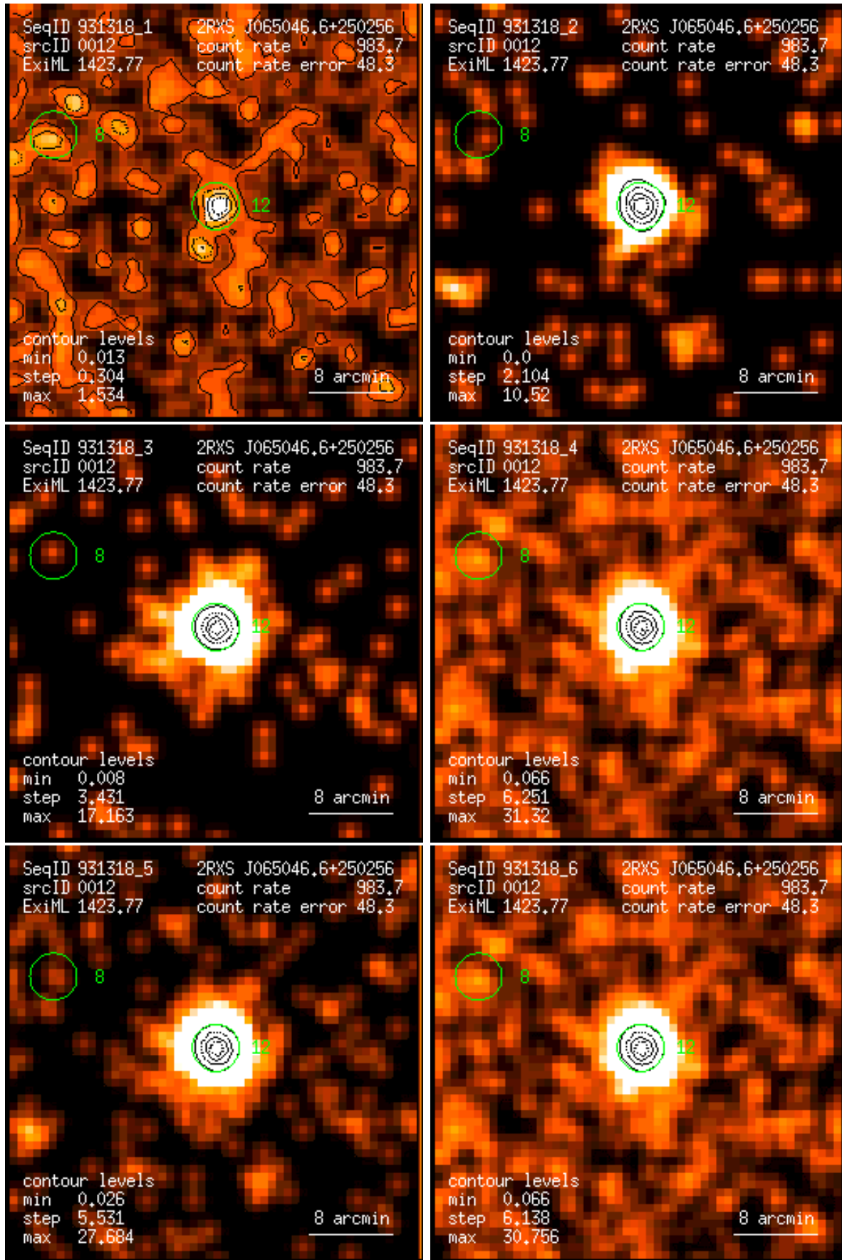
Figure 12: RASS 931318: detection 0012: band rate images, Gaussian filter: (1) PSPC channels 11 – 41, (2) 52 – 90, (3) 91 – 201, (4) 11 – 235, (5) 52 – 201, (6) 11 – 201. Broad band rates in counts/ks. Band rate contour levels in counts/ks/arcmin 2 .
