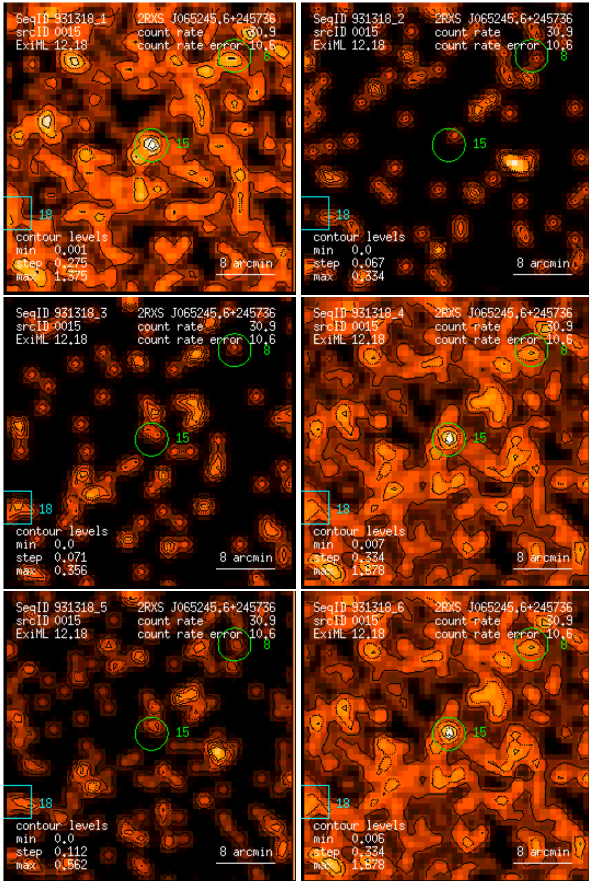
Figure 15: RASS 931318: detection 0015: band rate images, Gaussian filter: (1) PSPC channels 11 – 41, (2) 52 – 90, (3) 91 – 201, (4) 11 – 235, (5) 52 – 201, (6) 11 – 201. Broad band rates in counts/ks. Band rate contour levels in counts/ks/arcmin 2 .
