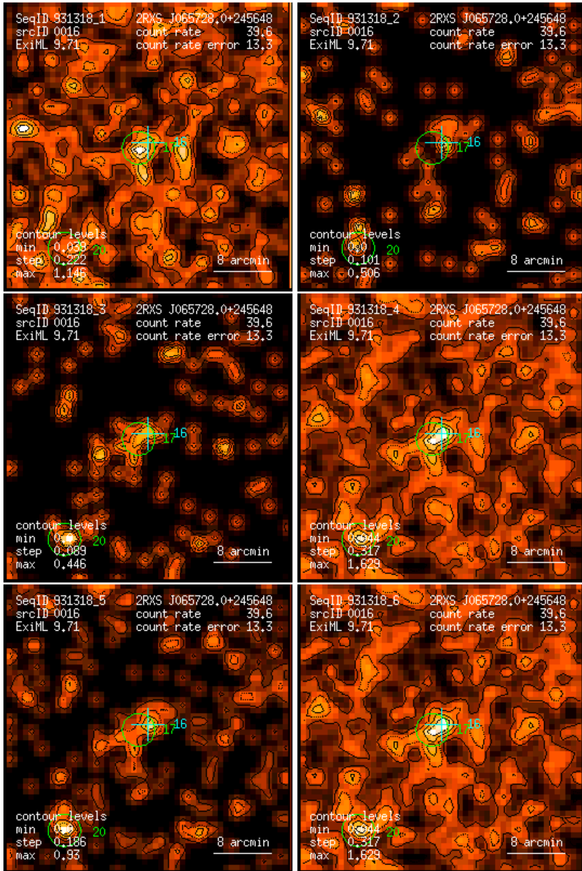
Figure 16: RASS 931318: detection 0016: band rate images, Gaussian filter: (1) PSPC channels 11 – 41, (2) 52 – 90, (3) 91 – 201, (4) 11 – 235, (5) 52 – 201, (6) 11 – 201. Broad band rates in counts/ks. Band rate contour levels in counts/ks/arcmin 2 .
