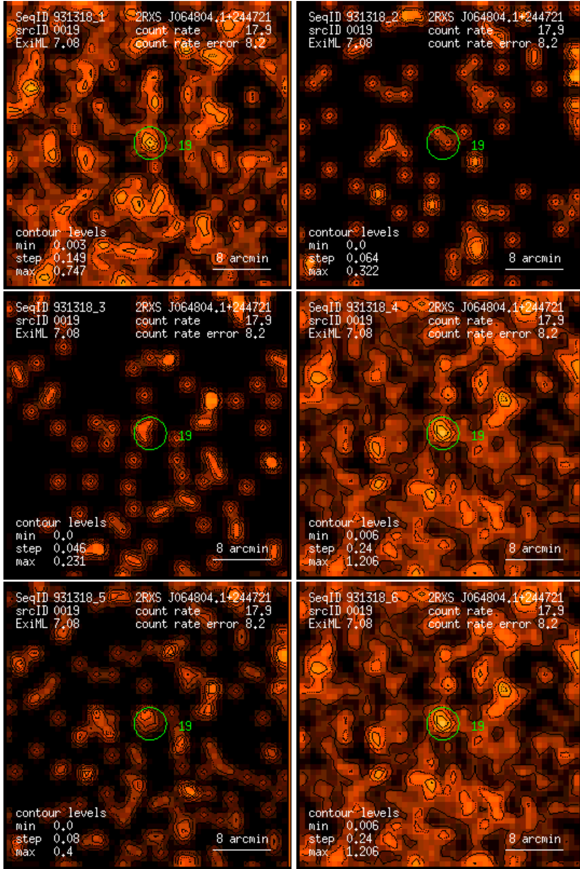
Figure 19: RASS 931318: detection 0019: band rate images, Gaussian filter: (1) PSPC channels 11 – 41, (2) 52 – 90, (3) 91 – 201, (4) 11 – 235, (5) 52 – 201, (6) 11 – 201. Broad band rates in counts/ks. Band rate contour levels in counts/ks/arcmin 2 .
