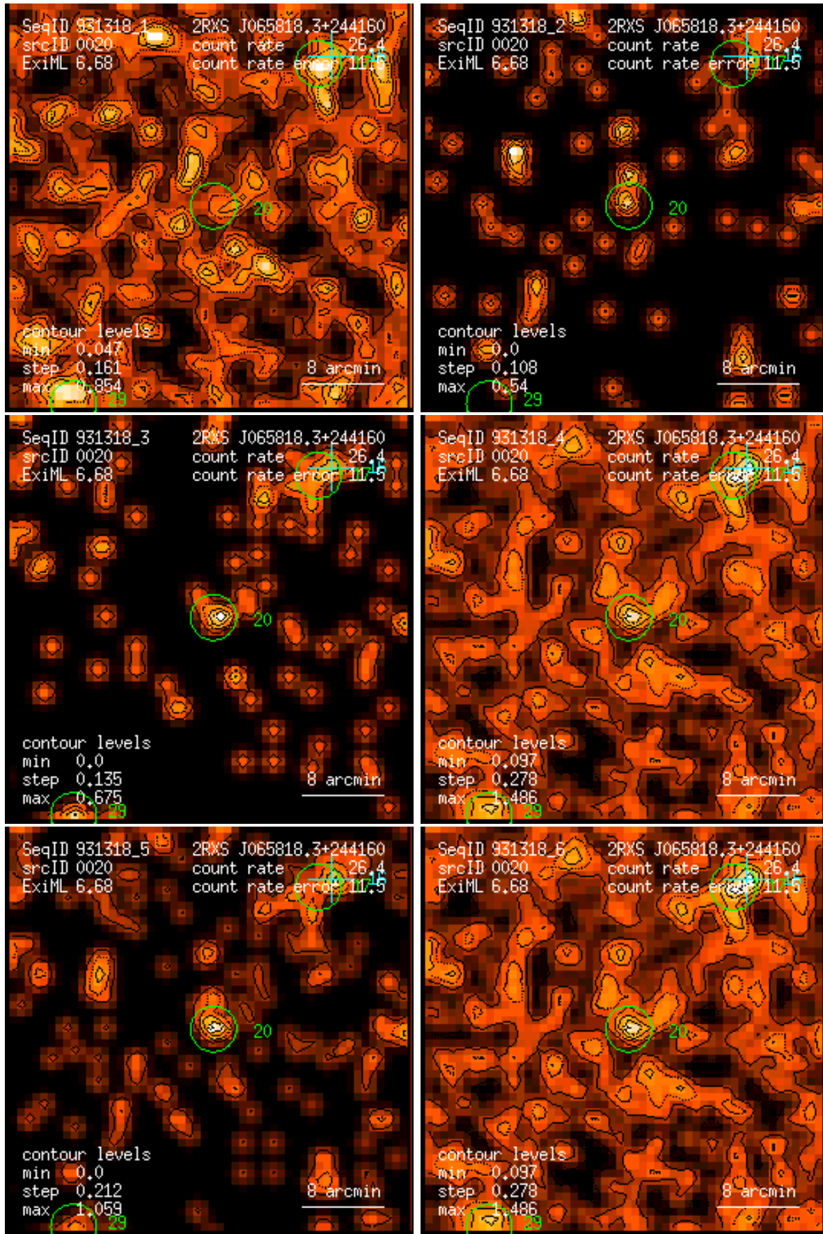
Figure 20: RASS 931318: detection 0020: band rate images, Gaussian filter: (1) PSPC channels 11 – 41, (2) 52 – 90, (3) 91 – 201, (4) 11 – 235, (5) 52 – 201, (6) 11 – 201. Broad band rates in counts/ks. Band rate contour levels in counts/ks/arcmin 2 .
