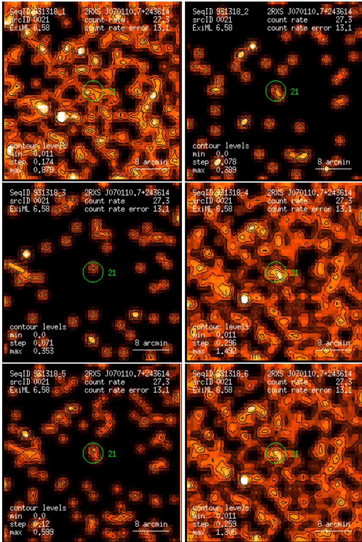
Figure 21: RASS 931318: detection 0021: band rate images, Gaussian filter: (1) PSPC channels 11 – 41, (2) 52 – 90, (3) 91 – 201, (4) 11 – 235, (5) 52 – 201, (6) 11 – 201. Broad band rates in counts/ks. Band rate contour levels in counts/ks/arcmin 2 .
