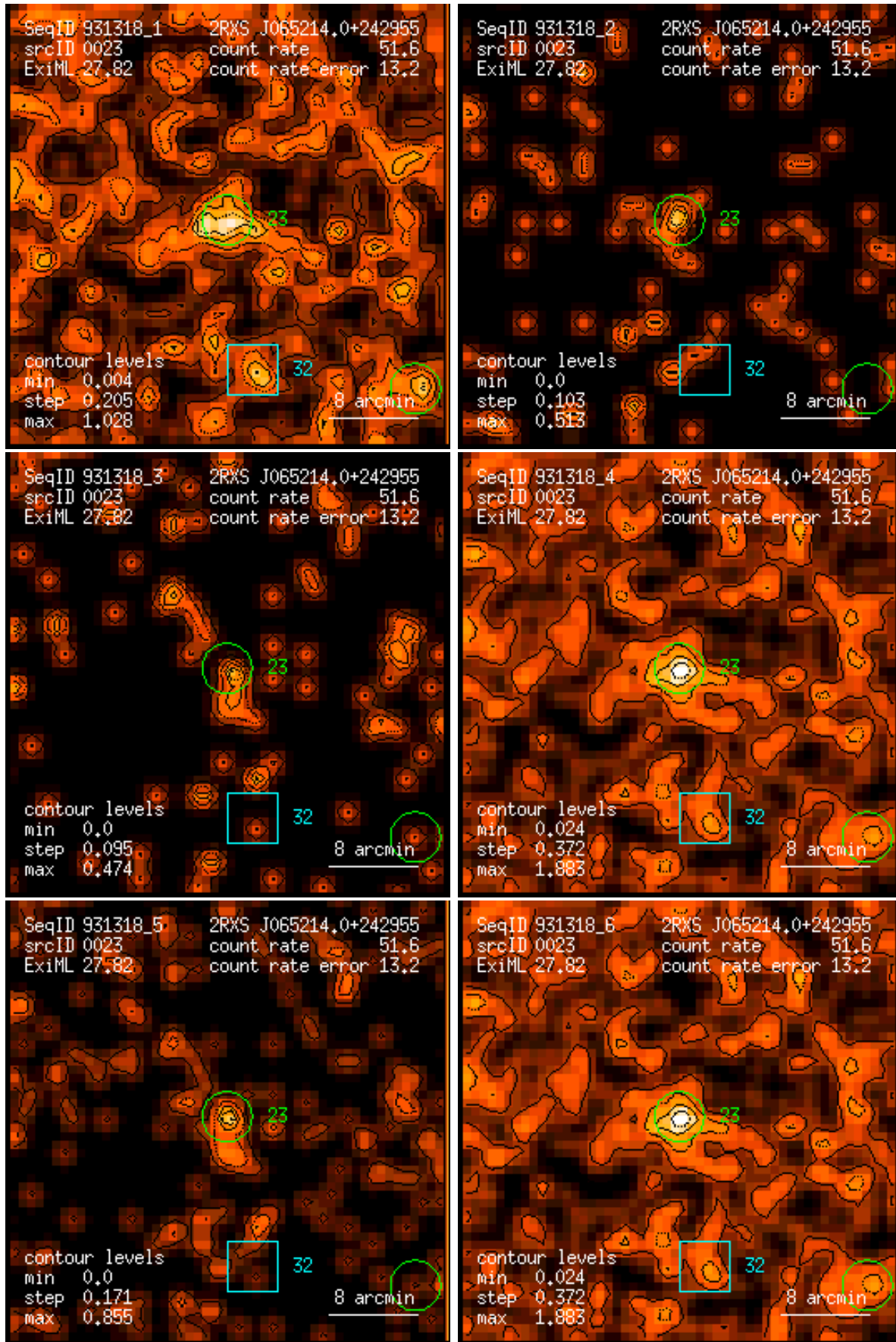
Figure 23: RASS 931318: detection 0023: band rate images, Gaussian filter: (1) PSPC channels 11 – 41, (2) 52 – 90, (3) 91 – 201, (4) 11 – 235, (5) 52 – 201, (6) 11 – 201. Broad band rates in counts/ks. Band rate contour levels in counts/ks/arcmin 2 .
