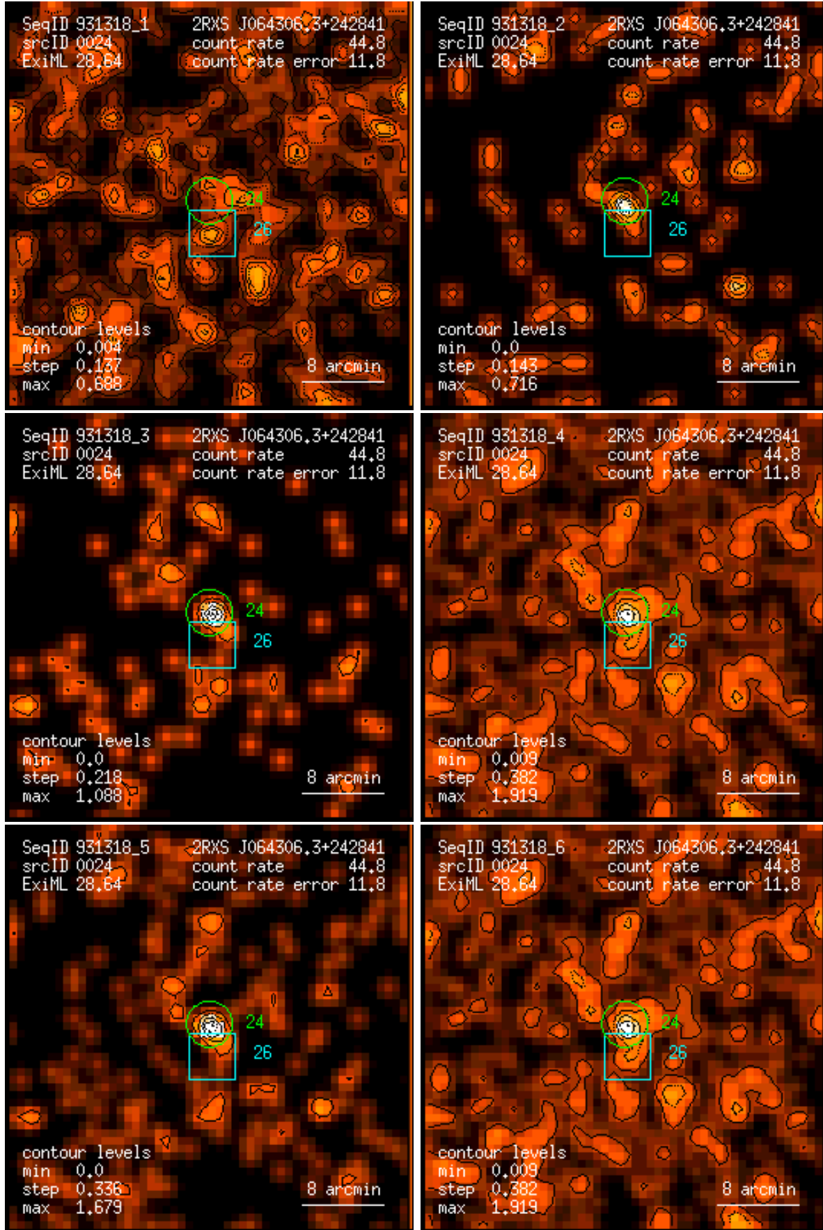
Figure 24: RASS 931318: detection 0024: band rate images, Gaussian filter: (1) PSPC channels 11 – 41, (2) 52 – 90, (3) 91 – 201, (4) 11 – 235, (5) 52 – 201, (6) 11 – 201. Broad band rates in counts/ks. Band rate contour levels in counts/ks/arcmin 2 .
