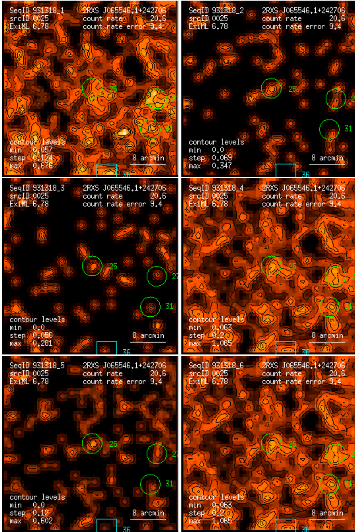
Figure 25: RASS 931318: detection 0025: band rate images, Gaussian filter: (1) PSPC channels 11 – 41, (2) 52 – 90, (3) 91 – 201, (4) 11 – 235, (5) 52 – 201, (6) 11 – 201. Broad band rates in counts/ks. Band rate contour levels in counts/ks/arcmin 2 .
