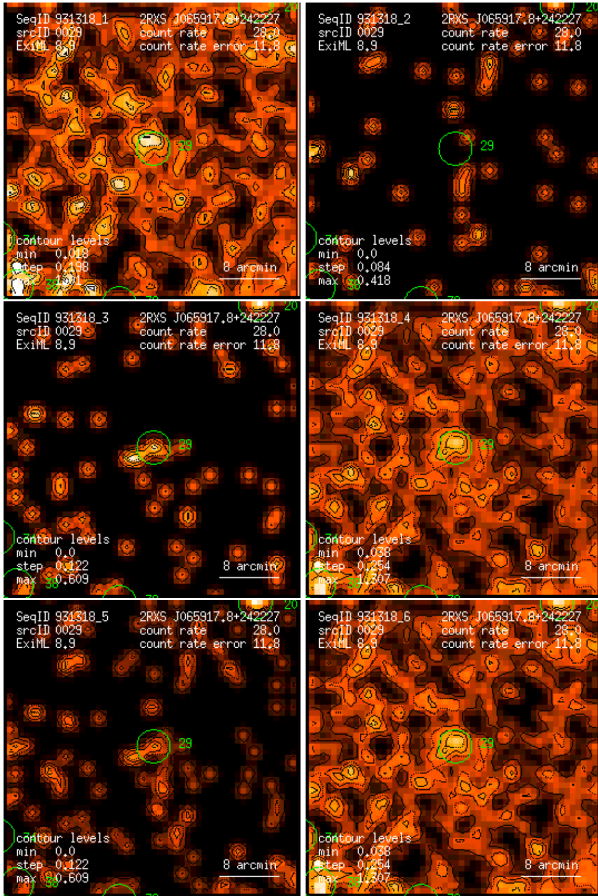
Figure 29: RASS 931318: detection 0029: band rate images, Gaussian filter: (1) PSPC channels 11 – 41, (2) 52 – 90, (3) 91 – 201, (4) 11 – 235, (5) 52 – 201, (6) 11 – 201. Broad band rates in counts/ks. Band rate contour levels in counts/ks/arcmin 2 .
