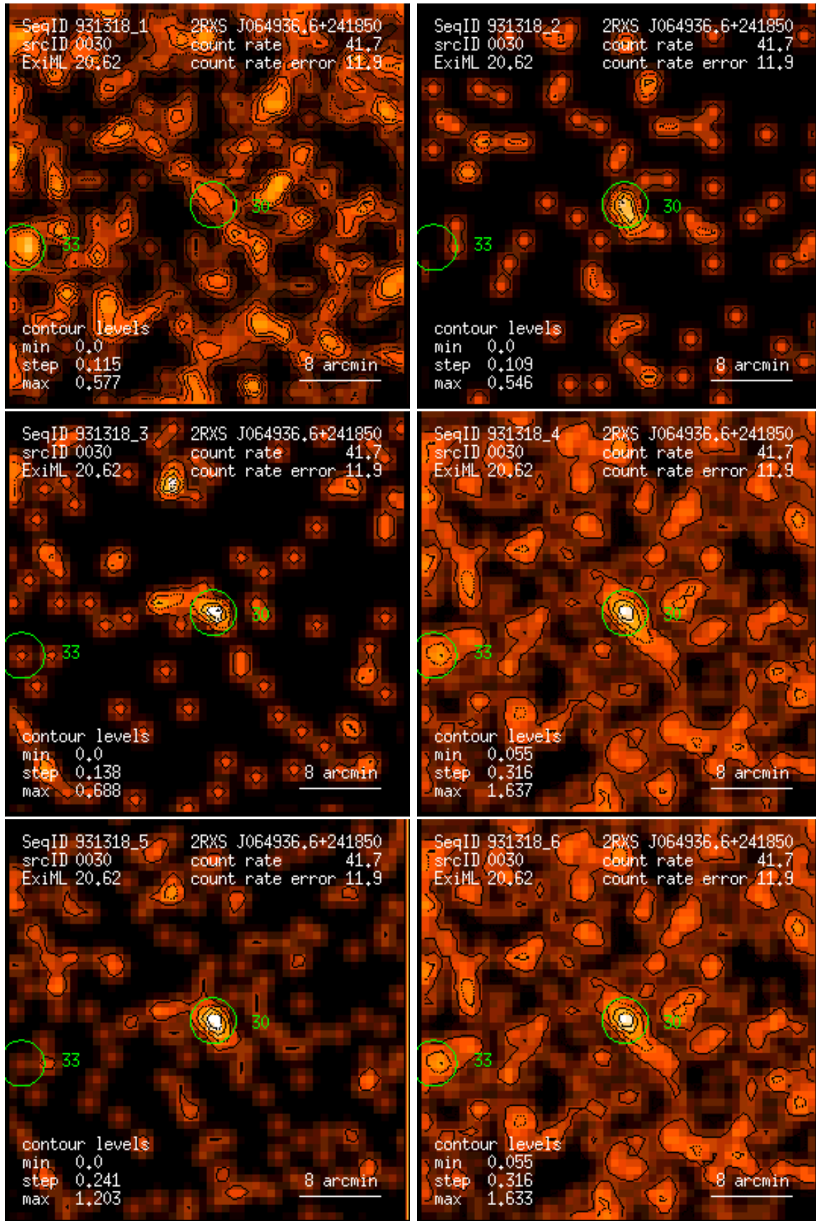
Figure 30: RASS 931318: detection 0030: band rate images, Gaussian filter: (1) PSPC channels 11 – 41, (2) 52 – 90, (3) 91 – 201, (4) 11 – 235, (5) 52 – 201, (6) 11 – 201. Broad band rates in counts/ks. Band rate contour levels in counts/ks/arcmin 2 .
