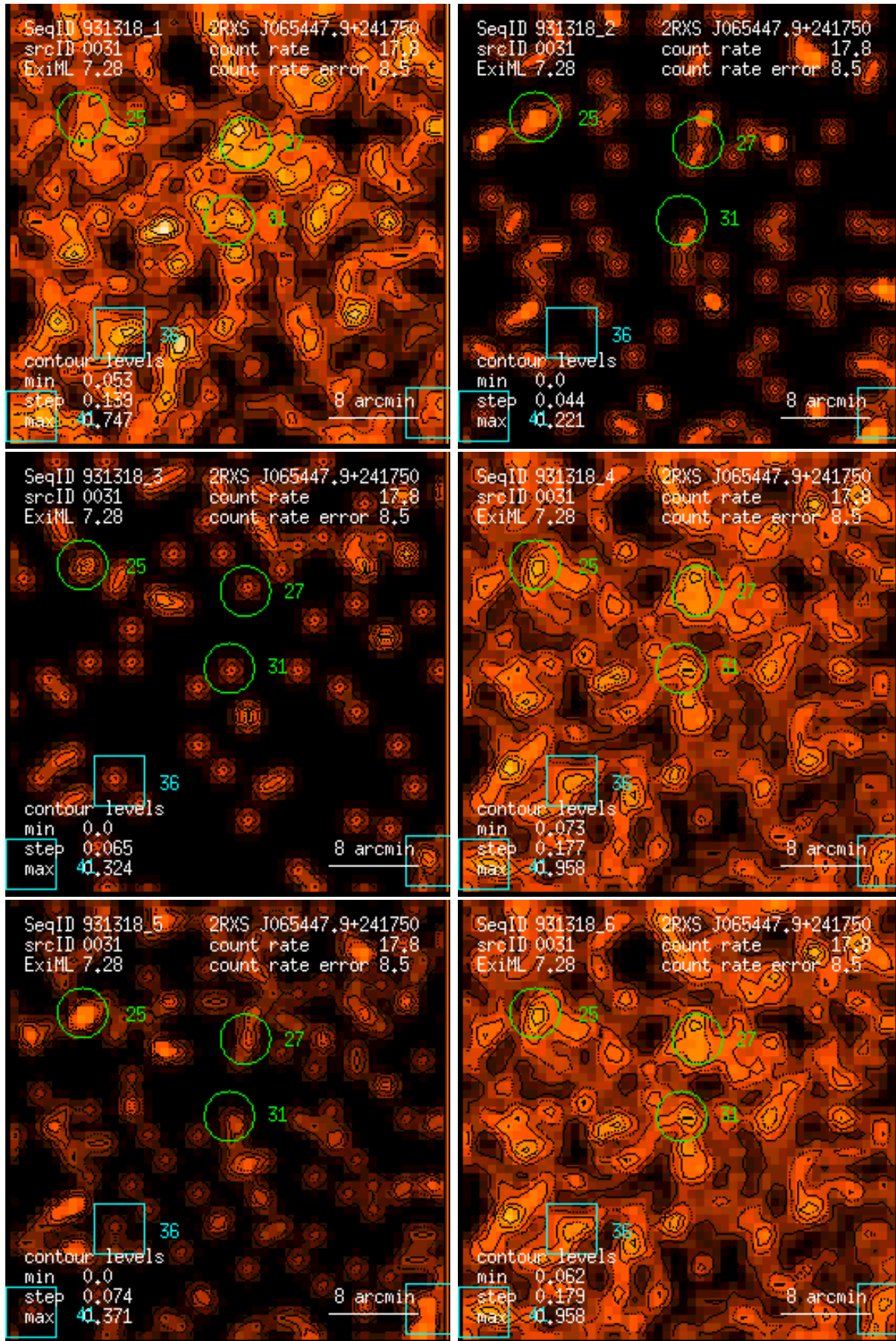
Figure 31: RASS 931318: detection 0031: band rate images, Gaussian filter: (1) PSPC channels 11 – 41, (2) 52 – 90, (3) 91 – 201, (4) 11 – 235, (5) 52 – 201, (6) 11 – 201. Broad band rates in counts/ks. Band rate contour levels in counts/ks/arcmin 2 .
