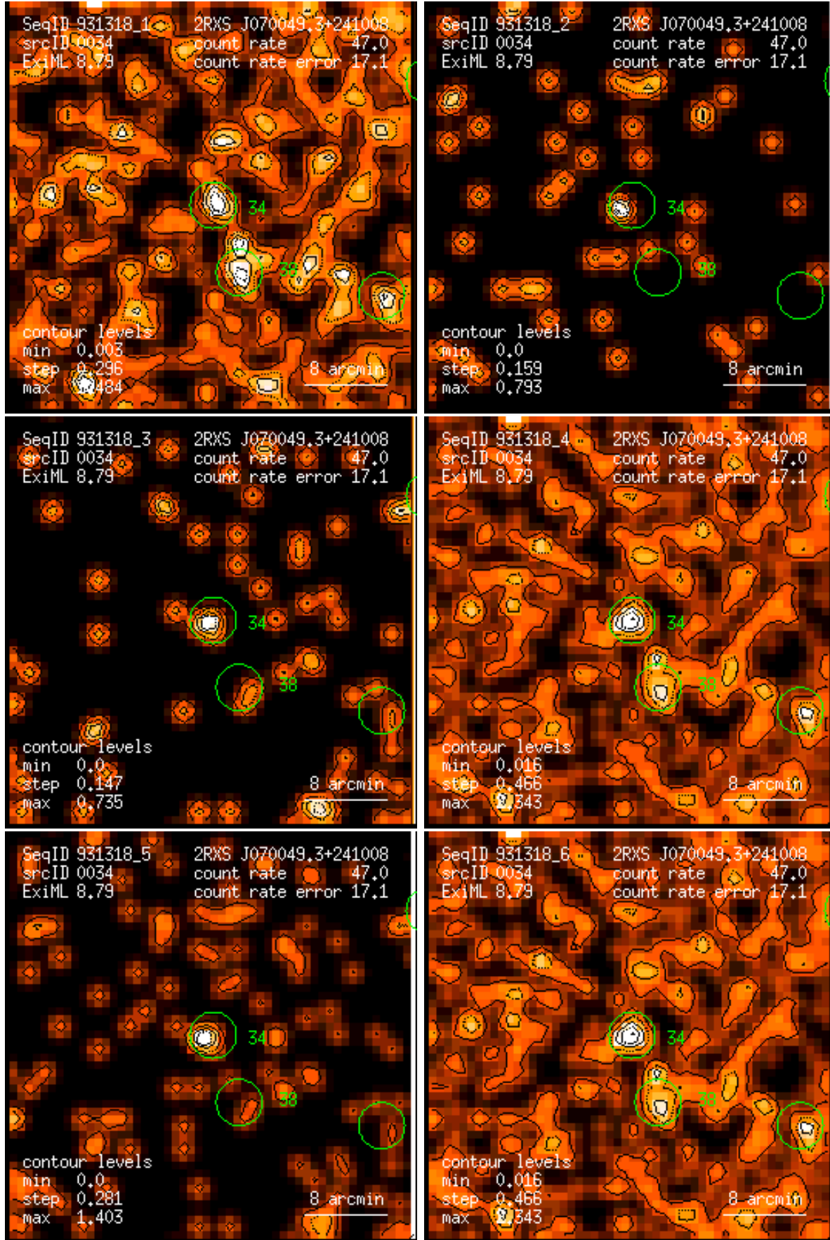
Figure 34: RASS 931318: detection 0034: band rate images, Gaussian filter: (1) PSPC channels 11 – 41, (2) 52 – 90, (3) 91 – 201, (4) 11 – 235, (5) 52 – 201, (6) 11 – 201. Broad band rates in counts/ks. Band rate contour levels in counts/ks/arcmin 2 .
