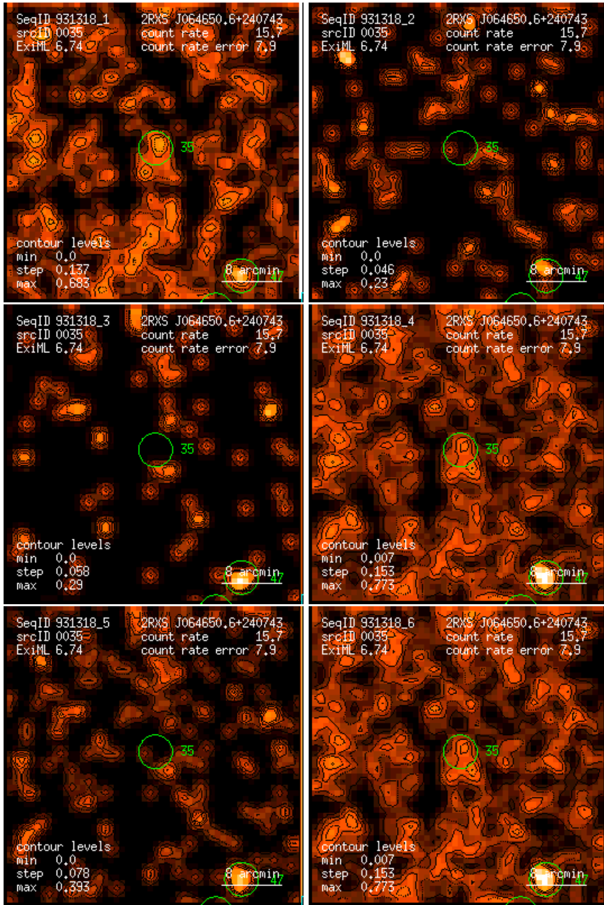
Figure 35: RASS 931318: detection 0035: band rate images, Gaussian filter: (1) PSPC channels 11 – 41, (2) 52 – 90, (3) 91 – 201, (4) 11 – 235, (5) 52 – 201, (6) 11 – 201. Broad band rates in counts/ks. Band rate contour levels in counts/ks/arcmin 2 .
