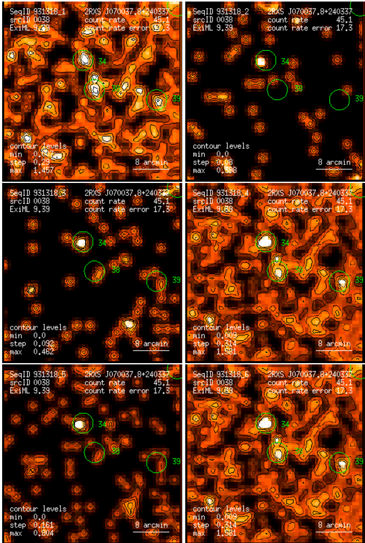
Figure 38: RASS 931318: detection 0038: band rate images, Gaussian filter: (1) PSPC channels 11 – 41, (2) 52 – 90, (3) 91 – 201, (4) 11 – 235, (5) 52 – 201, (6) 11 – 201. Broad band rates in counts/ks. Band rate contour levels in counts/ks/arcmin 2 .
