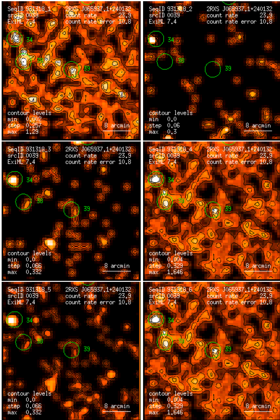
Figure 39: RASS 931318: detection 0039: band rate images, Gaussian filter: (1) PSPC channels 11 – 41, (2) 52 – 90, (3) 91 – 201, (4) 11 – 235, (5) 52 – 201, (6) 11 – 201. Broad band rates in counts/ks. Band rate contour levels in counts/ks/arcmin 2 .
