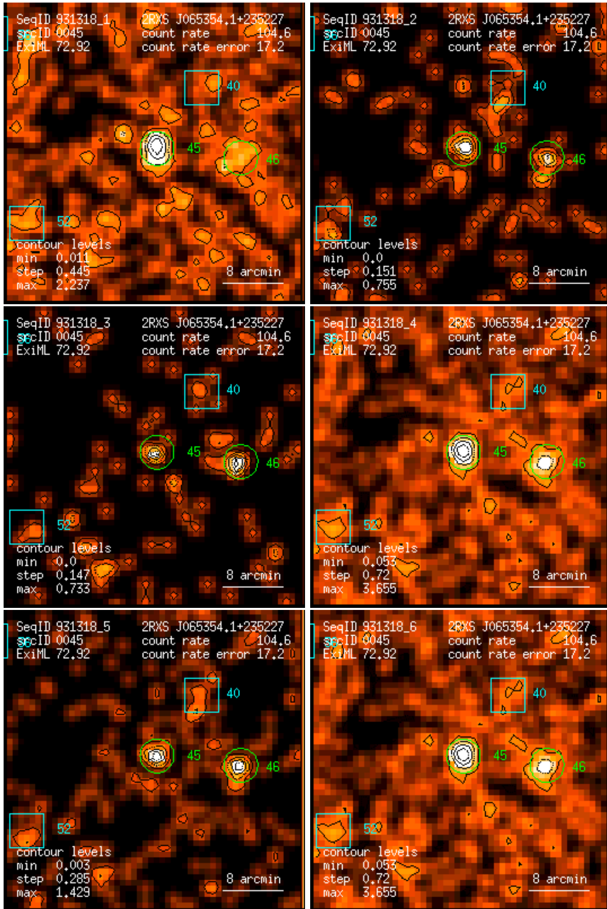
Figure 45: RASS 931318: detection 0045: band rate images, Gaussian filter: (1) PSPC channels 11 – 41, (2) 52 – 90, (3) 91 – 201, (4) 11 – 235, (5) 52 – 201, (6) 11 – 201. Broad band rates in counts/ks. Band rate contour levels in counts/ks/arcmin 2 .
