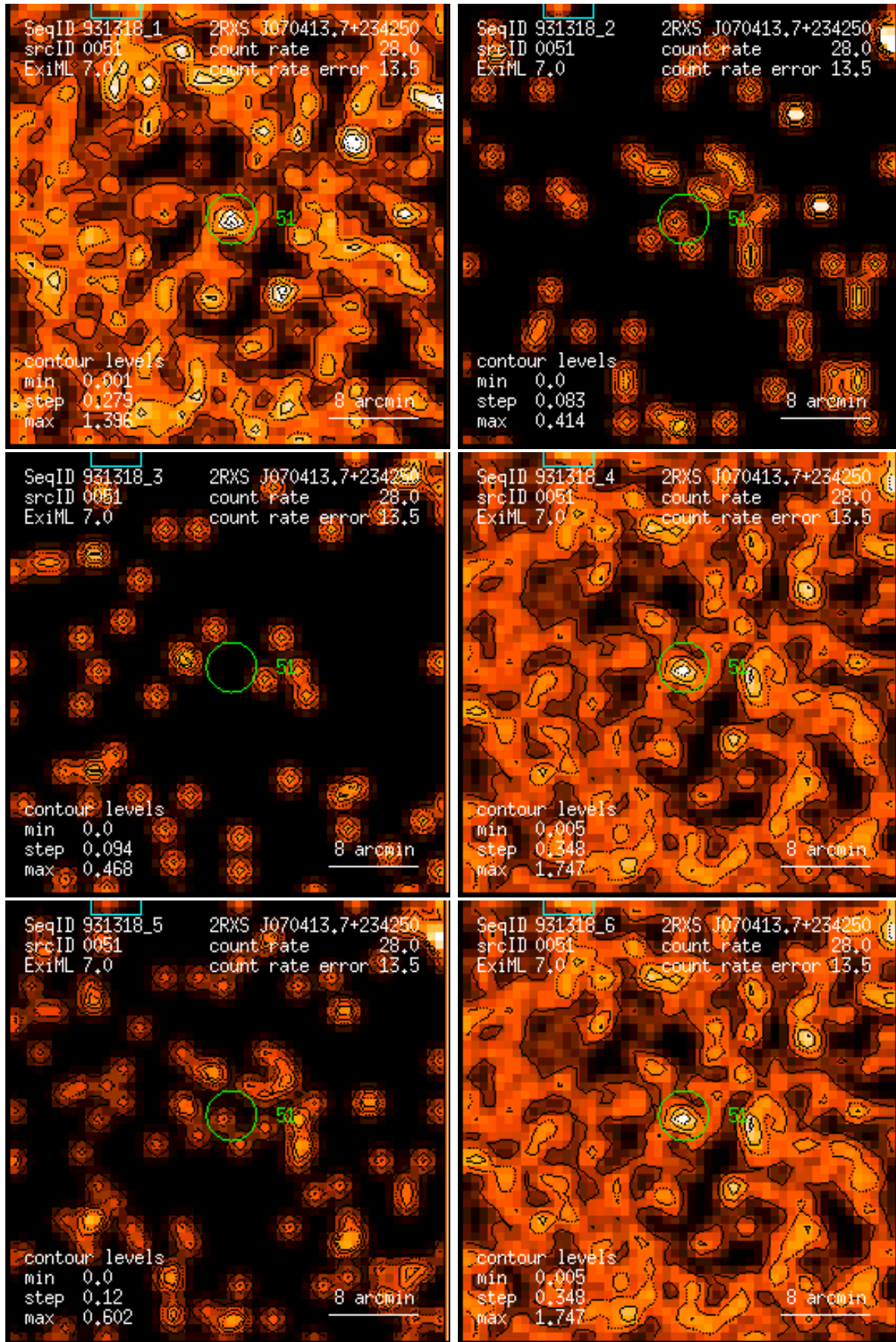
Figure 51: RASS 931318: detection 0051: band rate images, Gaussian filter: (1) PSPC channels 11 – 41, (2) 52 – 90, (3) 91 – 201, (4) 11 – 235, (5) 52 – 201, (6) 11 – 201. Broad band rates in counts/ks. Band rate contour levels in counts/ks/arcmin 2 .
