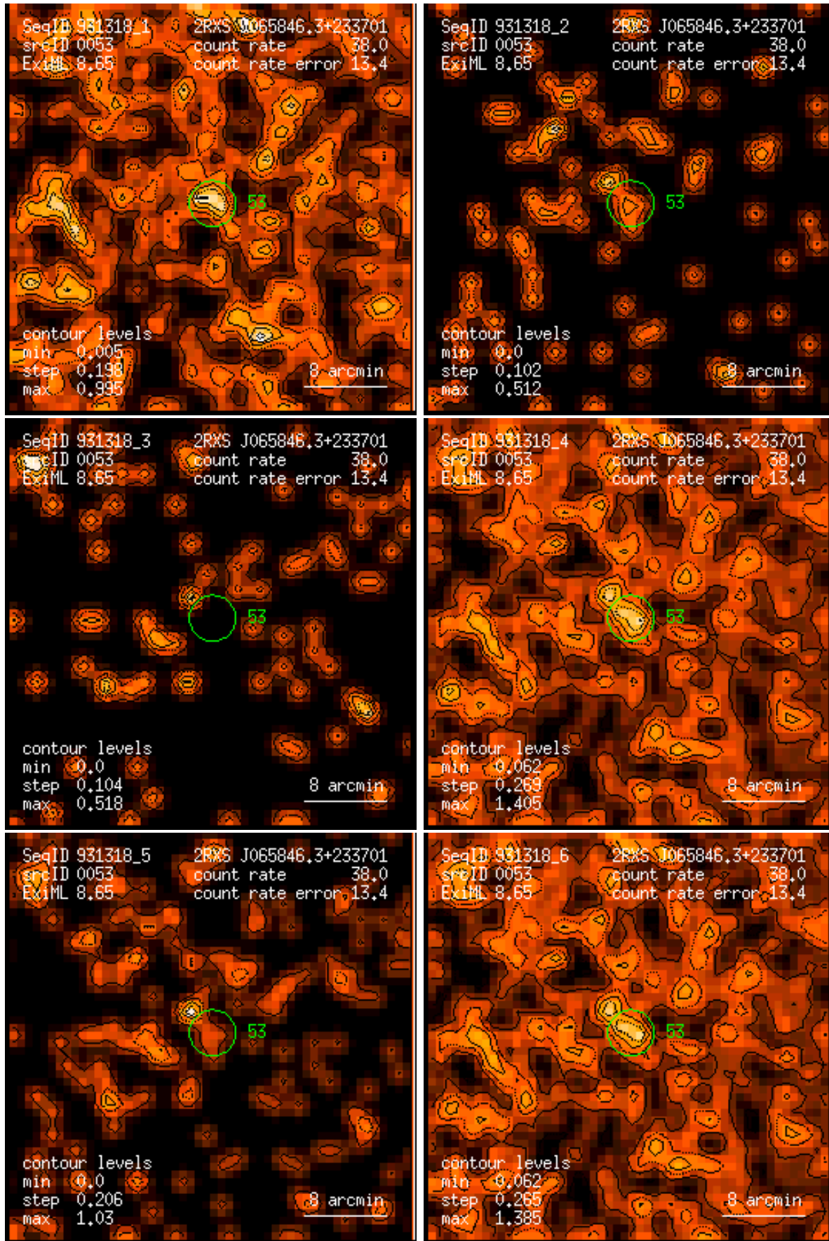
Figure 53: RASS 931318: detection 0053: band rate images, Gaussian filter: (1) PSPC channels 11 – 41, (2) 52 – 90, (3) 91 – 201, (4) 11 – 235, (5) 52 – 201, (6) 11 – 201. Broad band rates in counts/ks. Band rate contour levels in counts/ks/arcmin 2 .
