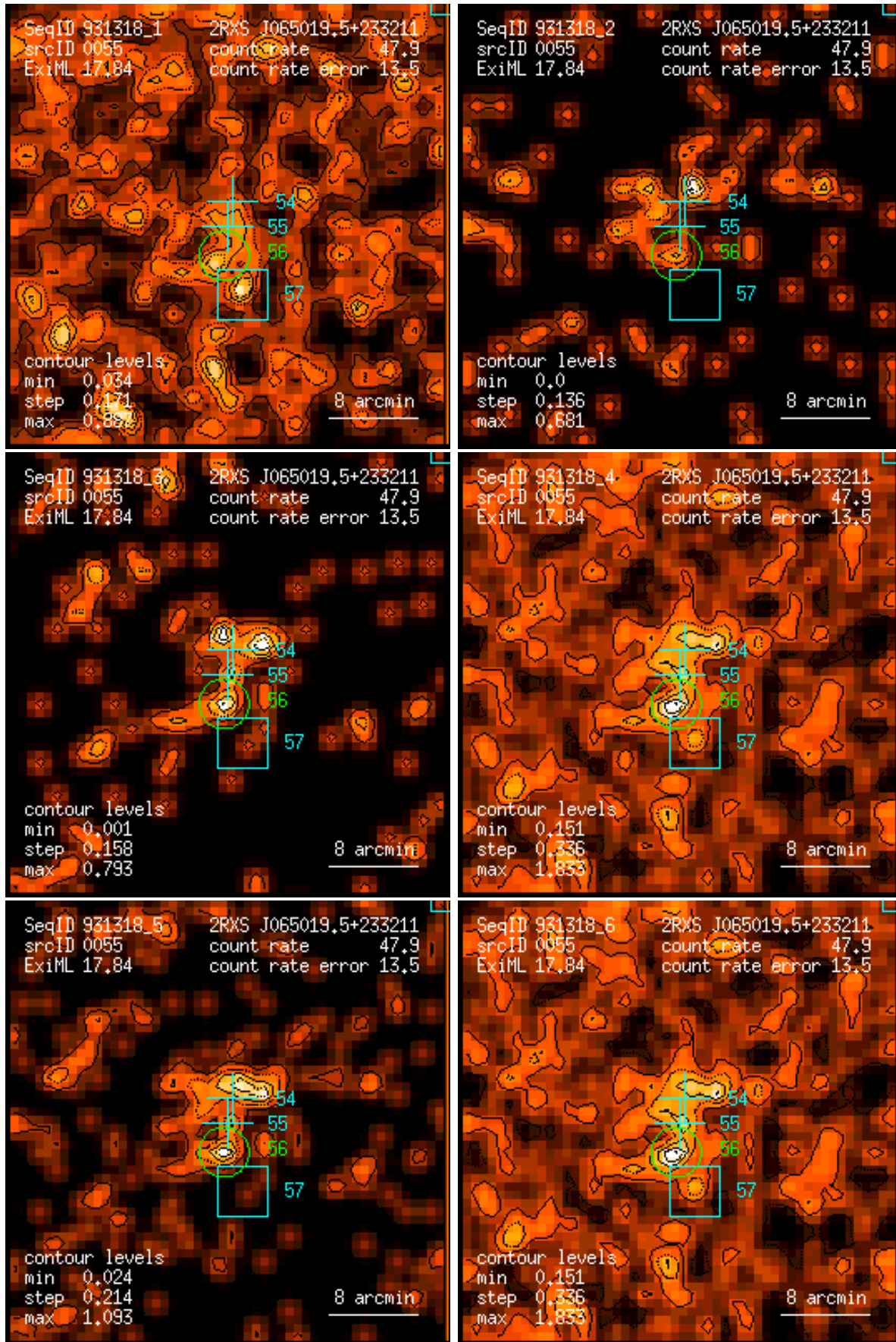
Figure 55: RASS 931318: detection 0055: band rate images, Gaussian filter: (1) PSPC channels 11 – 41, (2) 52 – 90, (3) 91 – 201, (4) 11 – 235, (5) 52 – 201, (6) 11 – 201. Broad band rates in counts/ks. Band rate contour levels in counts/ks/arcmin 2 .
