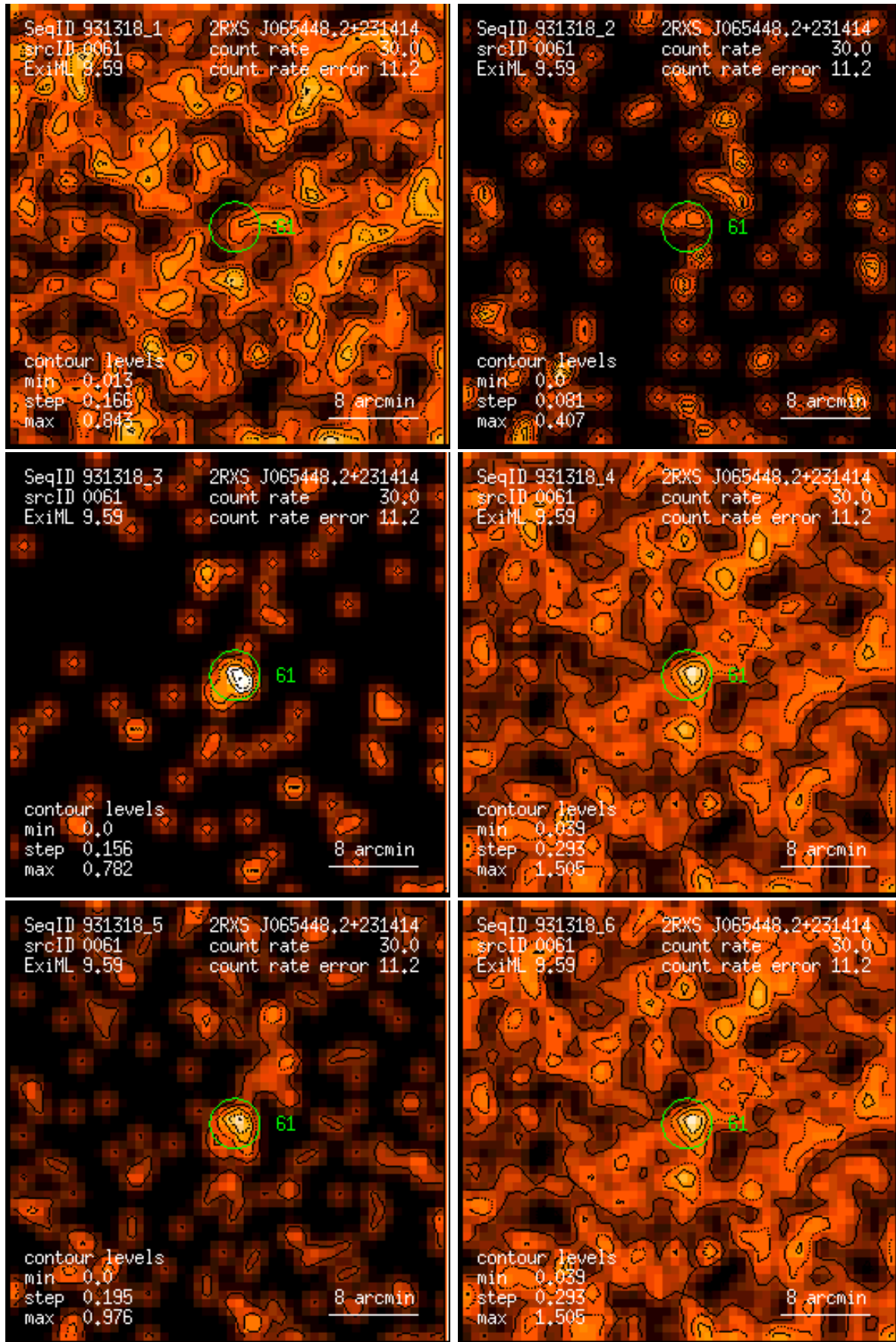
Figure 61: RASS 931318: detection 0061: band rate images, Gaussian filter: (1) PSPC channels 11 – 41, (2) 52 – 90, (3) 91 – 201, (4) 11 – 235, (5) 52 – 201, (6) 11 – 201. Broad band rates in counts/ks. Band rate contour levels in counts/ks/arcmin 2 .
