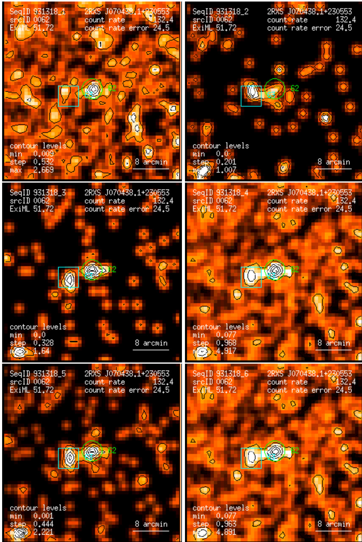
Figure 62: RASS 931318: detection 0062: band rate images, Gaussian filter: (1) PSPC channels 11 – 41, (2) 52 – 90, (3) 91 – 201, (4) 11 – 235, (5) 52 – 201, (6) 11 – 201. Broad band rates in counts/ks. Band rate contour levels in counts/ks/arcmin 2 .
