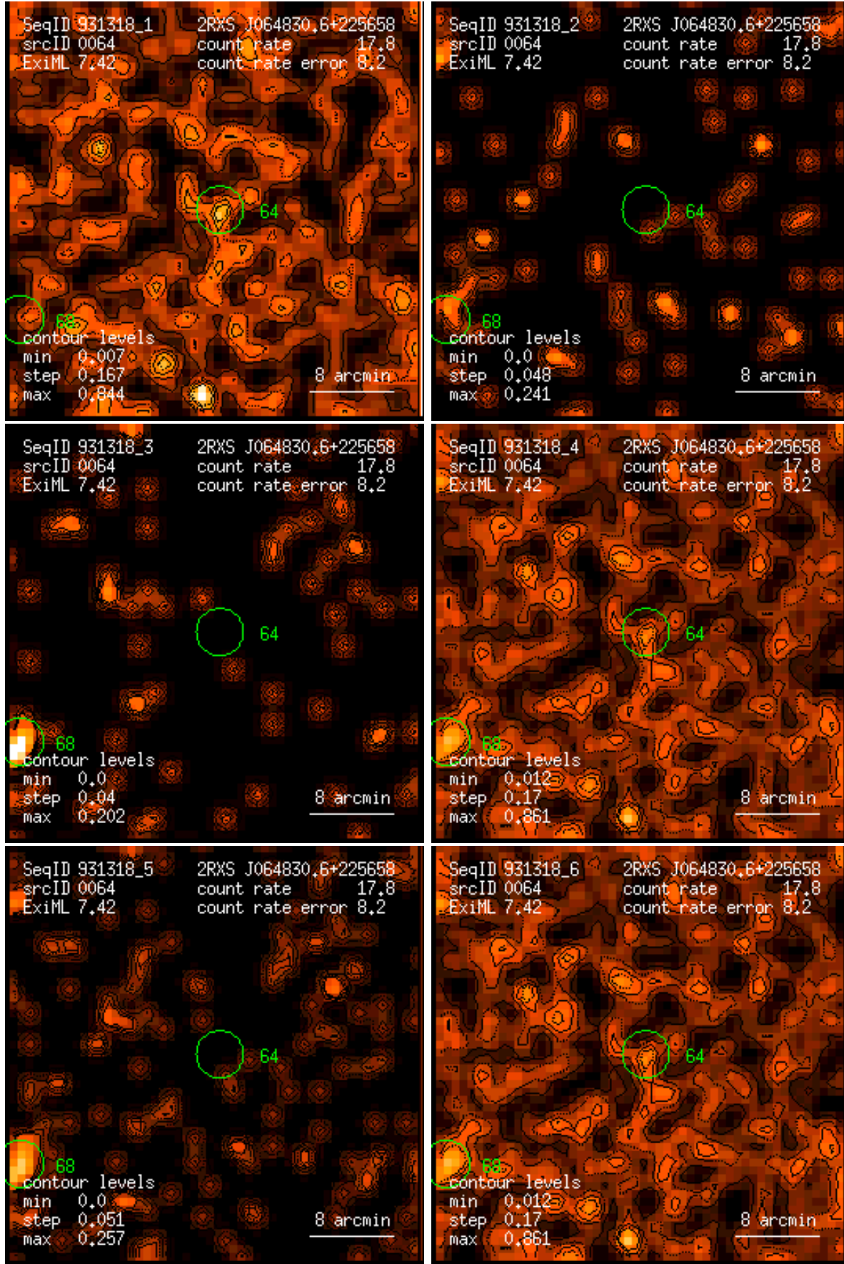
Figure 64: RASS 931318: detection 0064: band rate images, Gaussian filter: (1) PSPC channels 11 – 41, (2) 52 – 90, (3) 91 – 201, (4) 11 – 235, (5) 52 – 201, (6) 11 – 201. Broad band rates in counts/ks. Band rate contour levels in counts/ks/arcmin 2 .
