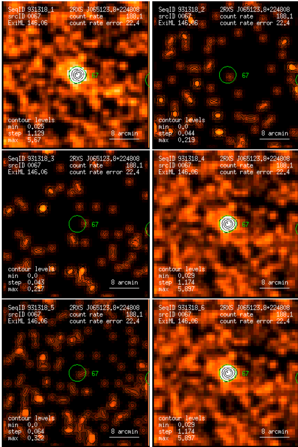
Figure 67: RASS 931318: detection 0067: band rate images, Gaussian filter: (1) PSPC channels 11 – 41, (2) 52 – 90, (3) 91 – 201, (4) 11 – 235, (5) 52 – 201, (6) 11 – 201. Broad band rates in counts/ks. Band rate contour levels in counts/ks/arcmin 2 .
