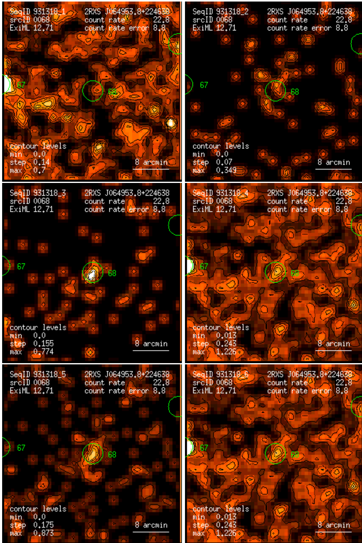
Figure 68: RASS 931318: detection 0068: band rate images, Gaussian filter: (1) PSPC channels 11 – 41, (2) 52 – 90, (3) 91 – 201, (4) 11 – 235, (5) 52 – 201, (6) 11 – 201. Broad band rates in counts/ks. Band rate contour levels in counts/ks/arcmin 2 .
